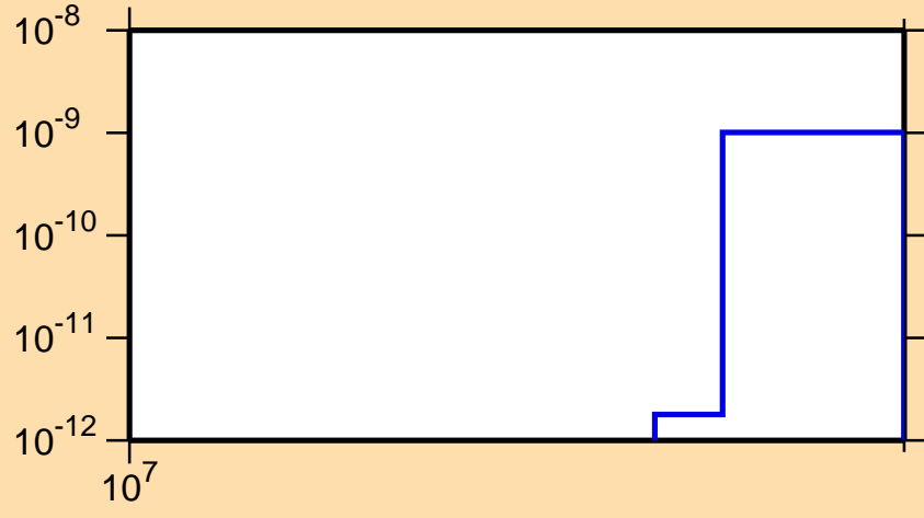
\sigma vs. E for ^{145}\text{Pr}(n,3n\alpha)
