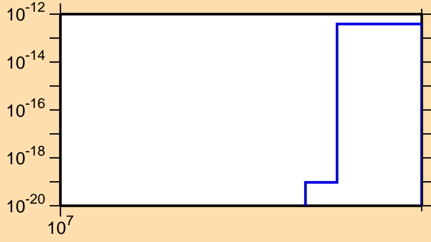
\sigma vs. E for ^{145}\text{Pr}(\text{mt 11})
