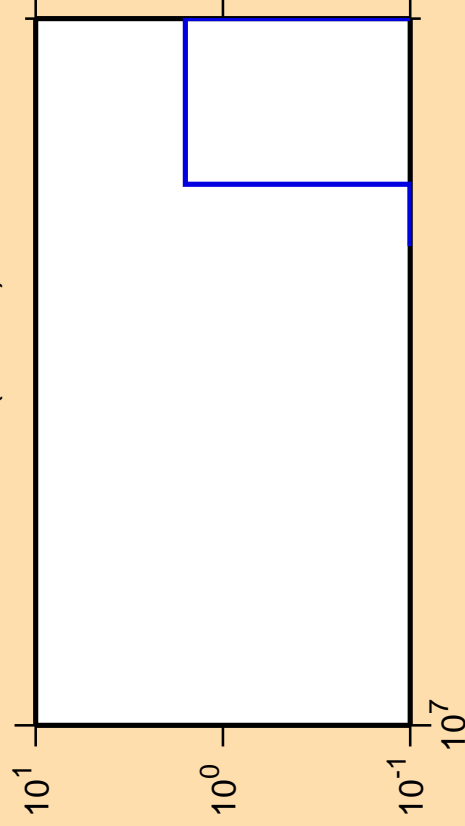
\Delta\sigma/\sigma vs. E for ^{145}\text{Pr}(\text{mt 11})
