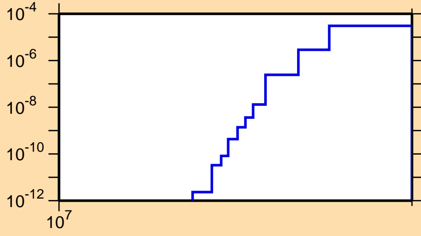
\sigma vs. E for ^{145}\text{Pr}(n,nt)
