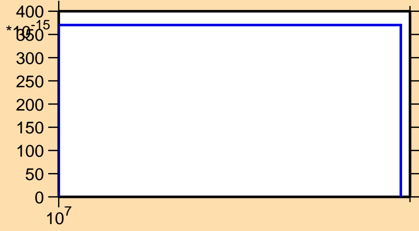
\sigma vs. E for ^{145}\text{Pr}(n,\text{He3})
