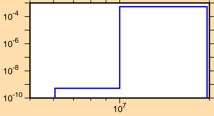
\sigma vs. E for ^{145}\text{Pr}(n,np)
