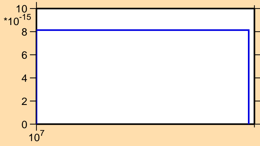
\sigma vs. E for ^{145}\text{Pr}(\text{mt117})
