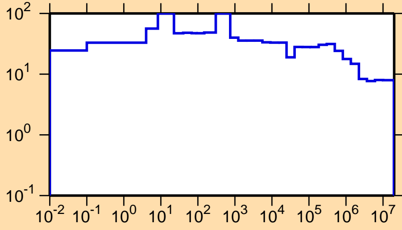
\Delta\sigma/\sigma vs. E for ^{145}\text{Pr}(n,\text{nonel.})
