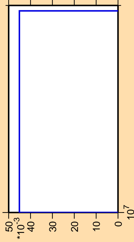
\Delta\sigma/\sigma vs. E for ^{145}\text{Pr}(\text{mt117})
