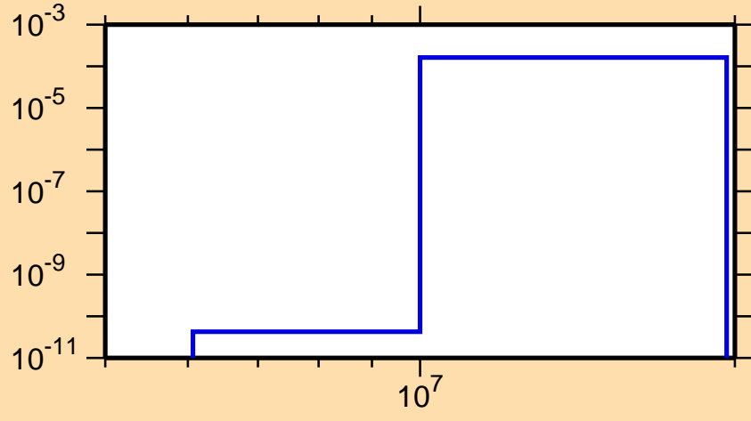
\sigma vs. E for ^{145}\text{Pr}(n,t)
