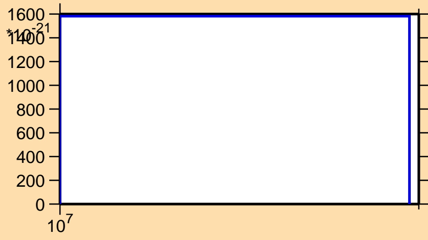
\sigma vs. E for ^{145}\text{Pr}(\text{mt } 42)
