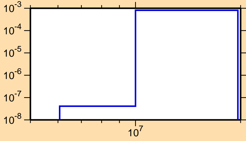
\sigma vs. E for ^{145}\text{Pr}(n,d)
