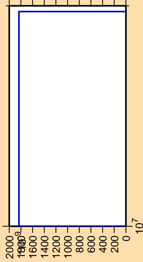
\Delta\sigma/\sigma vs. E for ^{145}\text{Pr}(\text{mt } 42)
