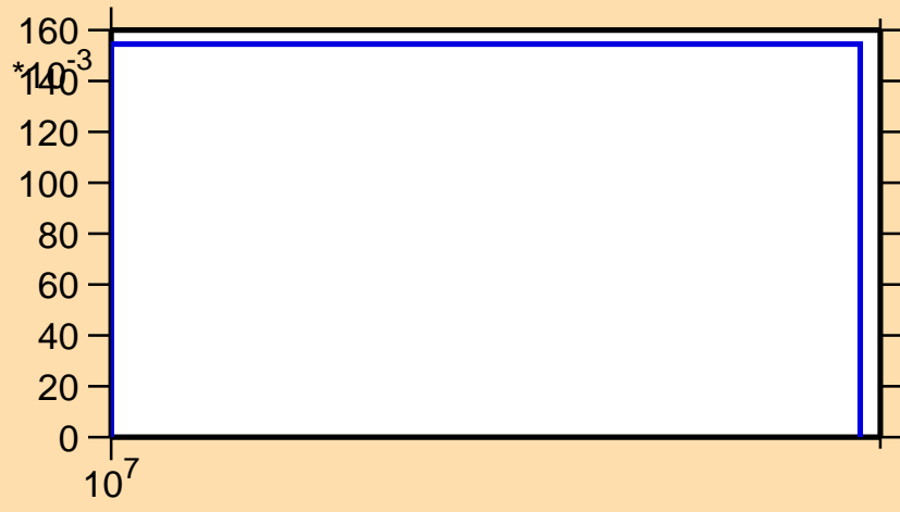
\sigma vs. E for ^{145}\text{Pr}(n,3n)
