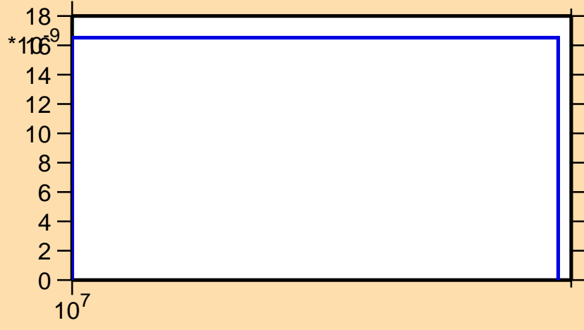
\sigma vs. E for ^{145}\text{Pr}(n,2np)
