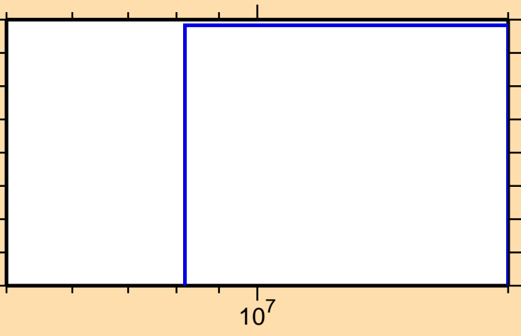
\sigma vs. E for ^{145}\text{Pr}(n,\text{He3})
