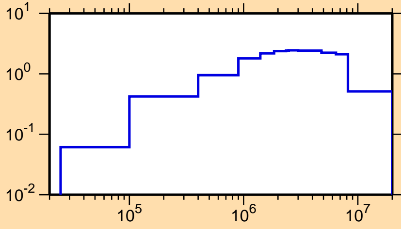
\sigma vs. E for ^{145}\text{Pr}(n,\text{inel.})
