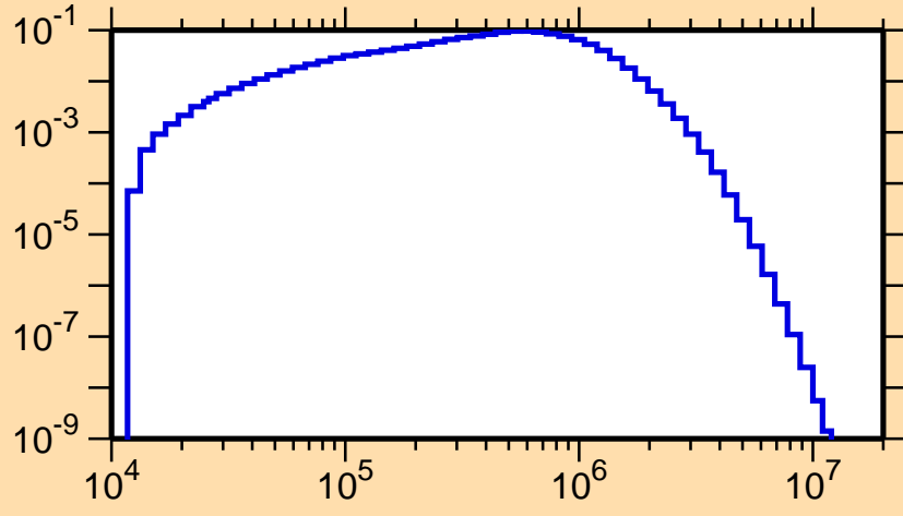
\sigma vs. E for ^{146}\text{Pr}(n,n_1)
