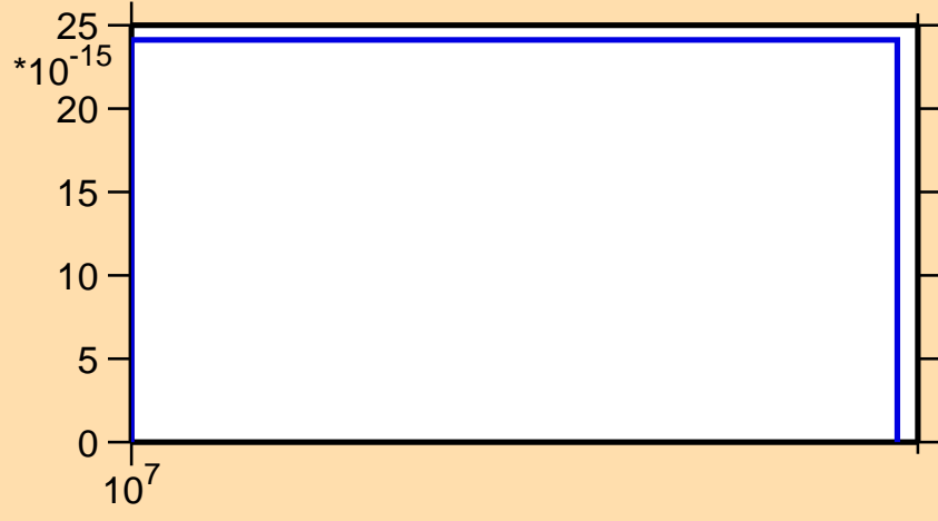
\sigma vs. E for ^{146}\text{Pr}(\text{mt } 11)
