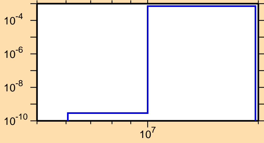
\sigma vs. E for ^{146}\text{Pr}(n,np)
