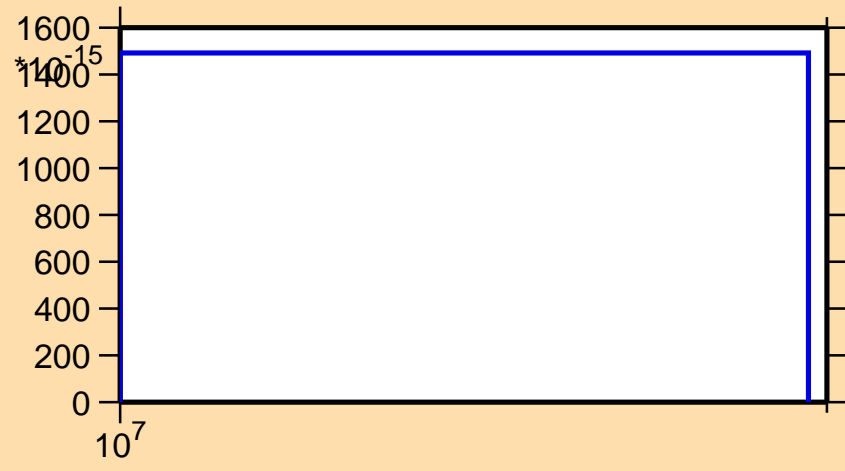
\sigma vs. E for ^{146}\text{Pr}(n,\text{He3})
