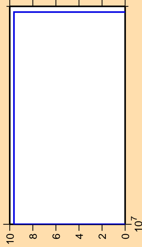
\Delta\sigma/\sigma vs. E for ^{146}\text{Pr}(n,\text{He3})
