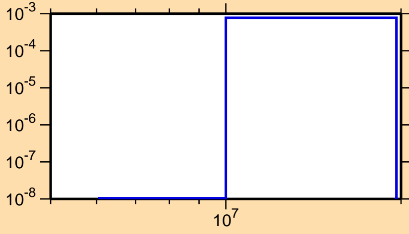
\sigma vs. E for ^{146}\text{Pr}(n,d)
