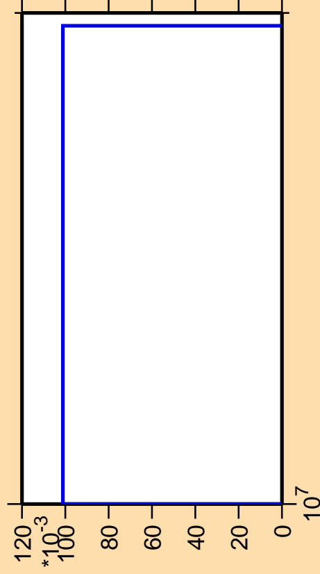
\Delta\sigma/\sigma vs. E for ^{146}\text{Pr}(\text{mt } 11)
