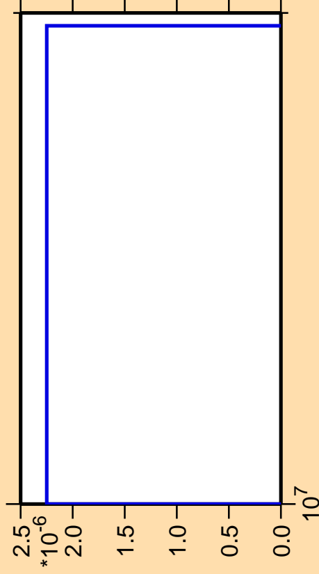
\Delta\sigma/\sigma vs. E for ^{146}\text{Pr}(\text{mt } 42)
