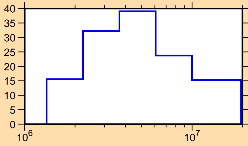
\Delta\sigma/\sigma vs. E for ^{146}\text{Pr}(n,\text{el.})
