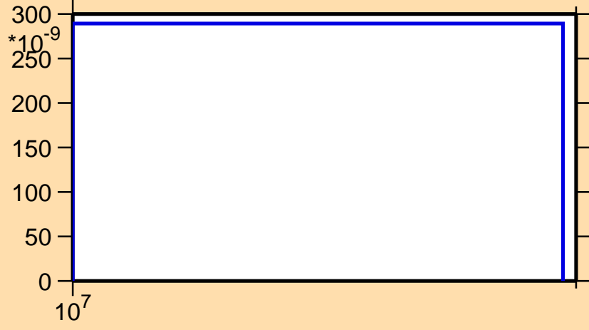
\sigma vs. E for ^{146}\text{Pr}(n,2np)
