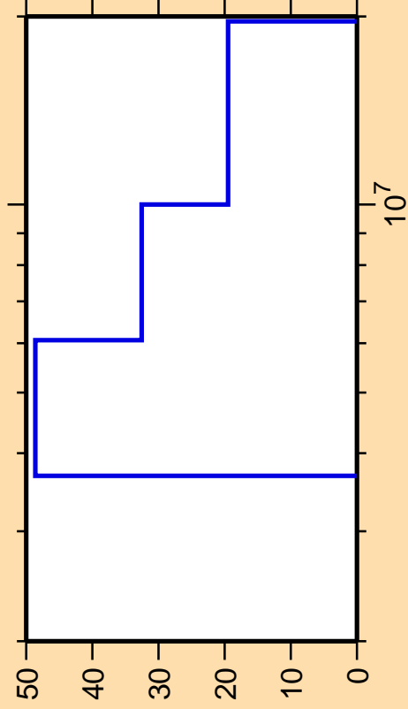
\Delta\sigma/\sigma vs. E for ^{146}\text{Pr}(n,2n)
