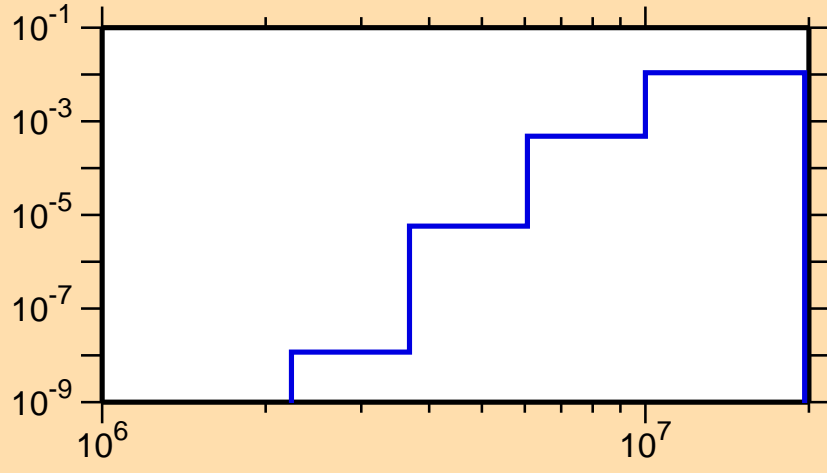
\sigma vs. E for ^{146}\text{Pr}(n,p)
