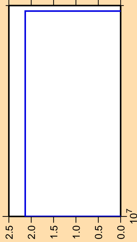
\Delta\sigma/\sigma vs. E for ^{146}\text{Pr}(n,p\alpha)
