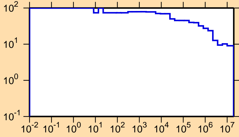
\Delta\sigma/\sigma vs. E for ^{146}\text{Pr}(n,\text{nonel.})
