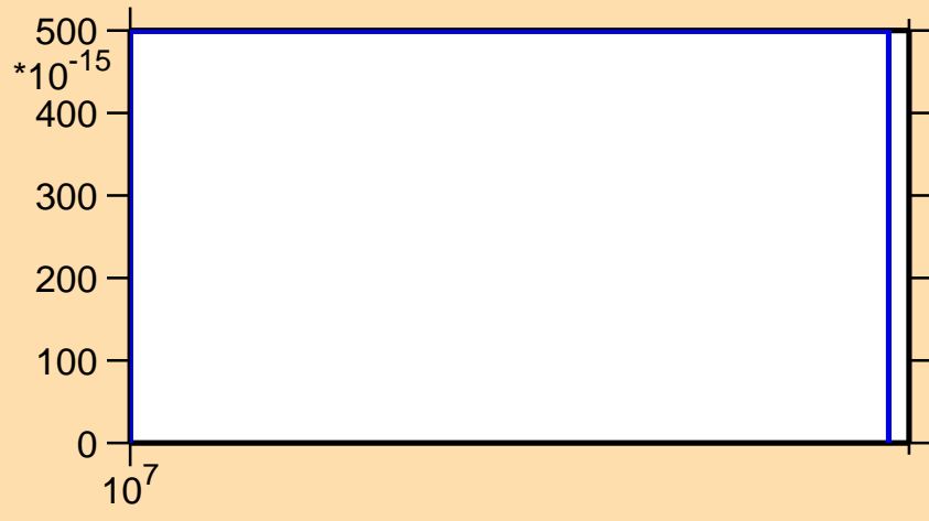
\sigma vs. E for ^{146}\text{Pr}(n,p\alpha)
