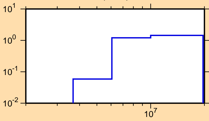
\sigma vs. E for ^{146}\text{Pr}(n,2n)
