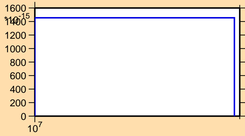
\sigma vs. E for ^{146}\text{Pr}(n,3n\alpha)
