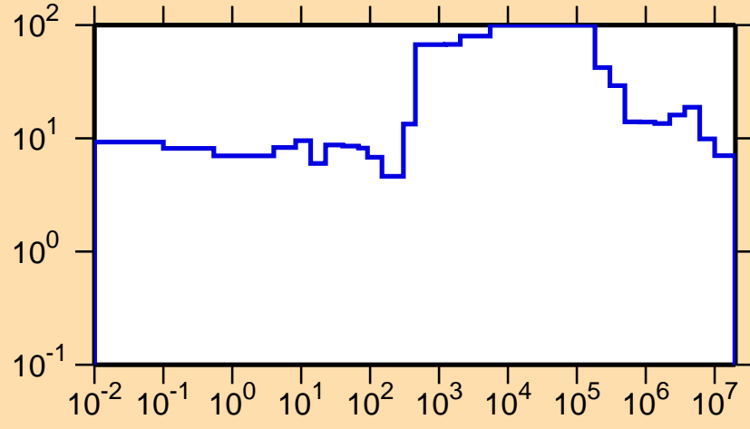
\Delta\sigma/\sigma vs. E for ^{146}\text{Pr}(n,\text{tot.})
