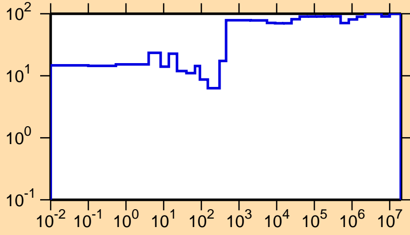
\Delta\sigma/\sigma vs. E for ^{146}\text{Pr}(n,\gamma)
