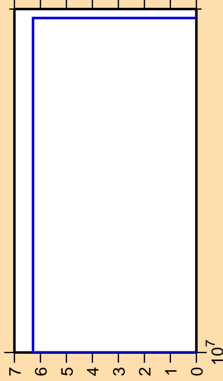
\Delta\sigma/\sigma vs. E for ^{146}\text{Pr}(n,3n\alpha)
