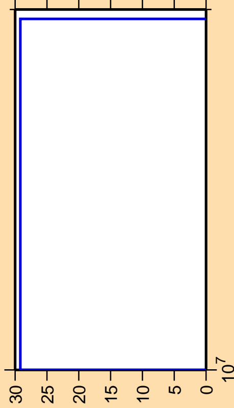
\Delta\sigma/\sigma vs. E for ^{146}\text{Pr}(n,3n)
