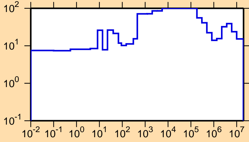
\Delta\sigma/\sigma vs. E for ^{146}\text{Pr}(n,\text{el.})
