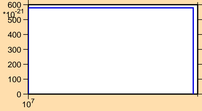
\sigma vs. E for ^{146}\text{Pr}(\text{mt } 42)
