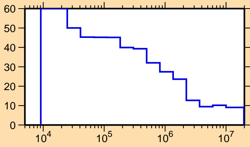
\Delta\sigma/\sigma vs. E for ^{146}\text{Pr}(n,\text{nonel.})
