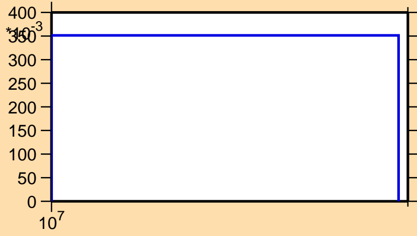
\sigma vs. E for ^{146}\text{Pr}(n,3n)
