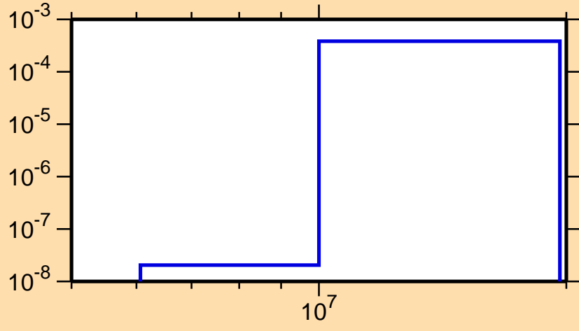
\sigma vs. E for ^{146}\text{Pr}(n,t)
