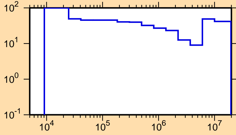
\Delta\sigma/\sigma vs. E for ^{146}\text{Pr}(n,\text{inel.})
