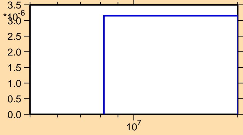
\sigma vs. E for ^{146}\text{Pr}(n,\text{nd})
