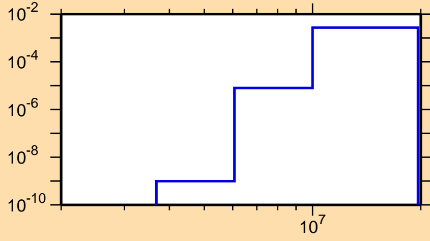
\sigma vs. E for ^{147}\text{Pr}(n,p)
