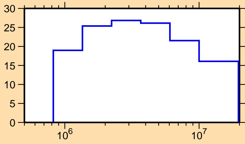
\Delta\sigma/\sigma vs. E for ^{147}\text{Pr}(n, el.)
