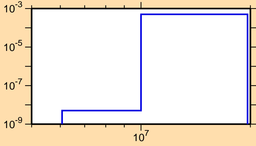
\sigma vs. E for ^{147}\text{Pr}(n,d)
