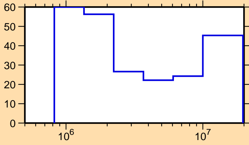
\Delta\sigma/\sigma vs. E for ^{147}\text{Pr}(n,n\text{cont.})
