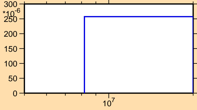
\sigma vs. E for ^{147}\text{Pr}(n,np)
