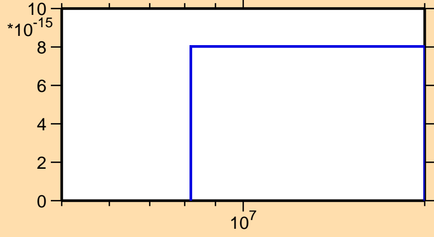
\sigma vs. E for ^{147}\text{Pr}(\text{mt } 11)
