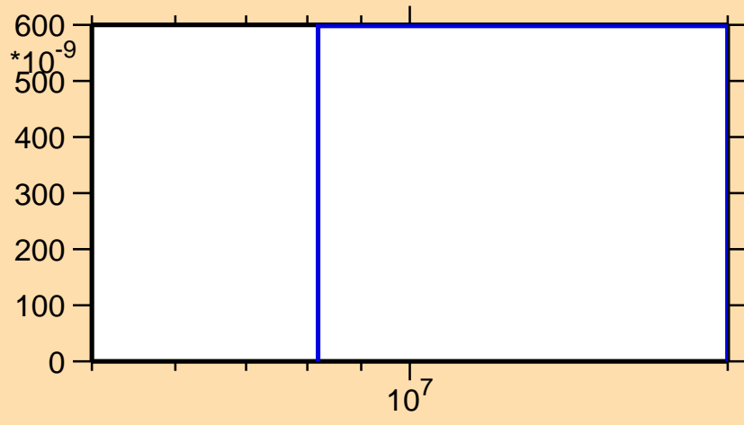
\sigma vs. E for ^{147}\text{Pr}(n,nt)
