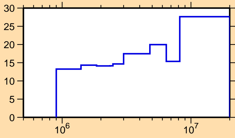
\Delta\sigma/\sigma vs. E for ^{147}\text{Pr}(n,\text{inel.})
