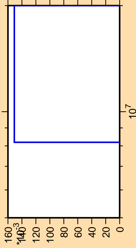
\Delta\sigma/\sigma vs. E for ^{147}\text{Pr}(n,\text{He3})
