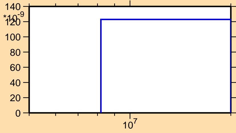
\sigma vs. E for ^{147}\text{Pr}(n,\text{nd})
