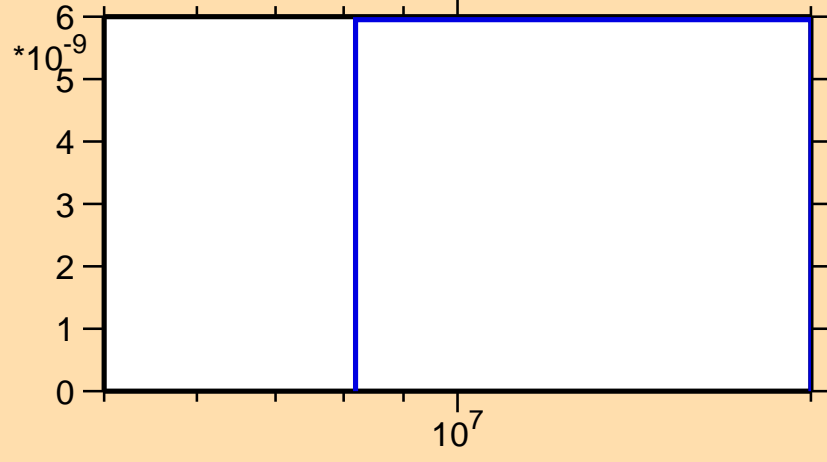
\sigma vs. E for ^{147}\text{Pr}(n,2np)
