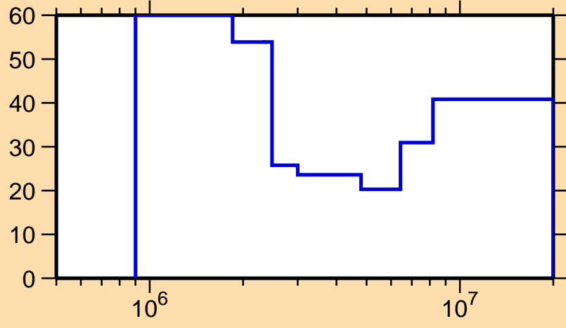
\Delta\sigma/\sigma vs. E for ^{147}\text{Pr}(n,n\text{cont.})
