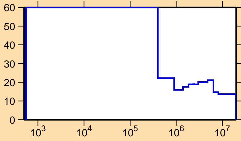
\Delta\sigma/\sigma vs. E for ^{147}\text{Pr}(n,\text{tot.})
