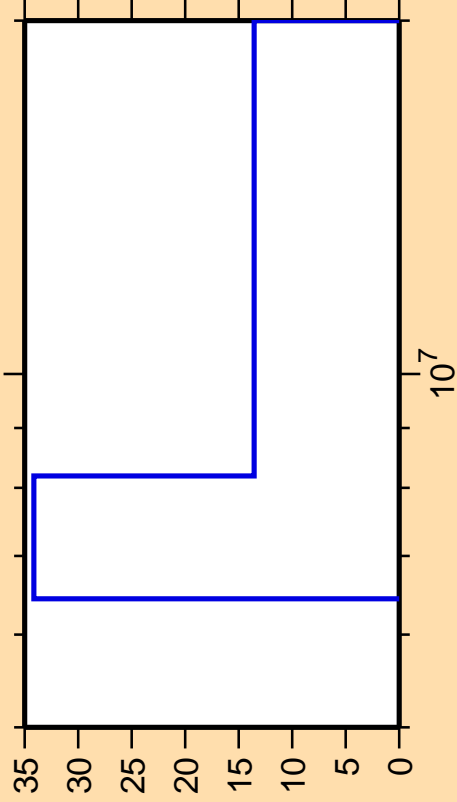
\Delta\sigma/\sigma vs. E for ^{147}\text{Pr}(n,2n)
