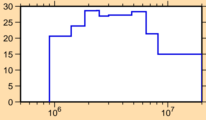
\Delta\sigma/\sigma vs. E for ^{147}\text{Pr}(n, \text{el.})
