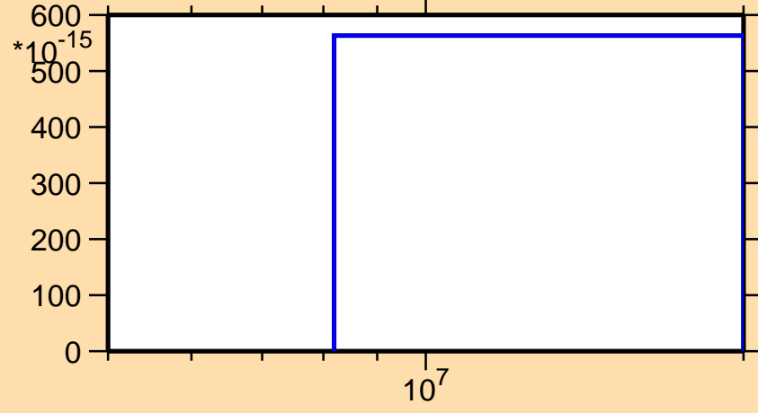
\sigma vs. E for ^{147}\text{Pr}(n,3n\alpha)
