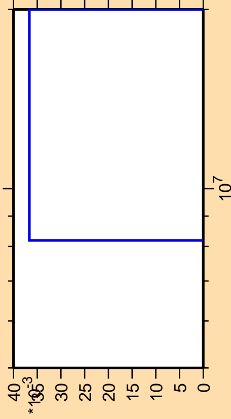
\Delta\sigma/\sigma vs. E for ^{147}\text{Pr}(\text{mt } 11)
