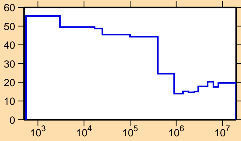
\Delta\sigma/\sigma vs. E for ^{147}\text{Pr}(n,\text{nonel.})
