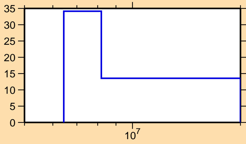
\Delta\sigma/\sigma vs. E for ^{147}\text{Pr}(n,2n)
