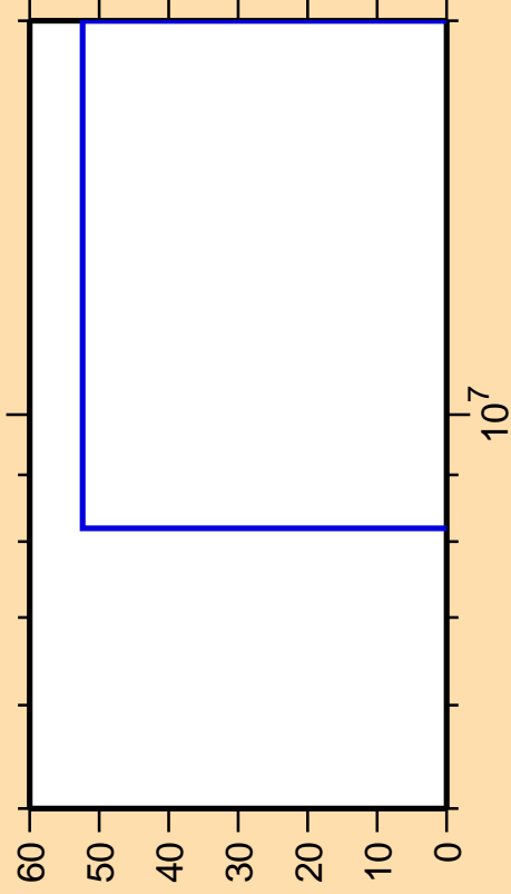
\Delta\sigma/\sigma vs. E for ^{147}\text{Pr}(n,3n)
