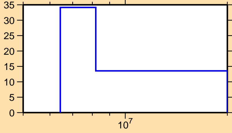
\Delta\sigma/\sigma vs. E for ^{147}\text{Pr}(n,2n)
