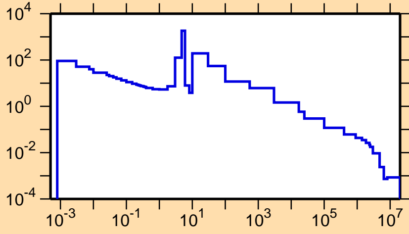
\sigma vs. E for ^{147}\text{Pr}(n,\gamma)
