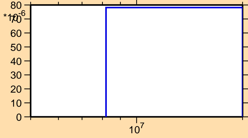
\sigma vs. E for ^{147}\text{Pr}(n,t)
