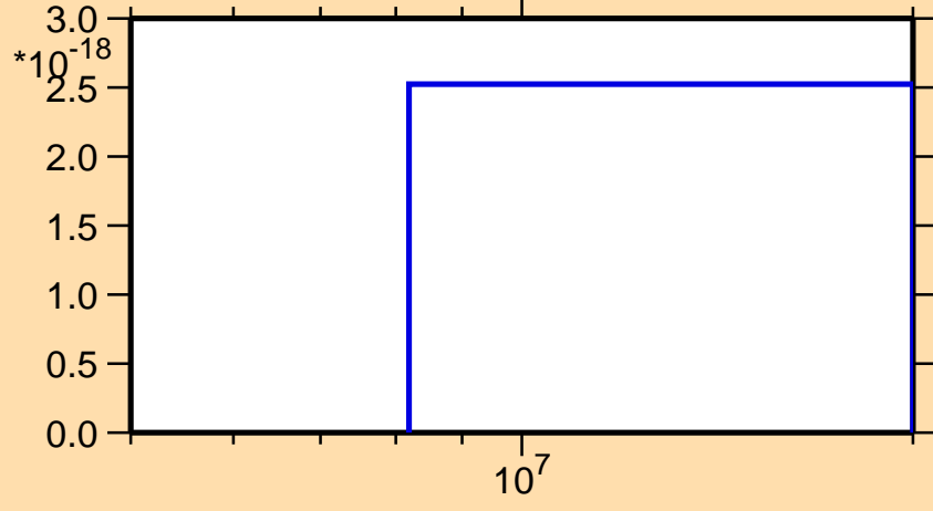
\sigma vs. E for ^{147}\text{Pr}(\text{mt } 42)
