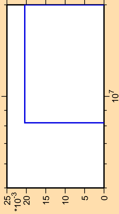
\Delta\sigma/\sigma vs. E for ^{147}\text{Pr}(n,p\alpha)
