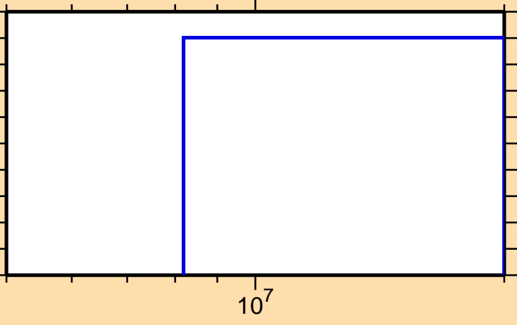
\sigma vs. E for ^{147}\text{Pr}(n,\text{He3})
