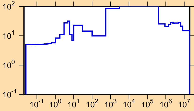
\Delta\sigma/\sigma vs. E for ^{147}\text{Pr}(n,\text{el.})
