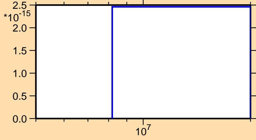
\sigma vs. E for ^{147}\text{Pr}(n,p\alpha)
