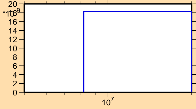
\sigma vs. E for ^{147}\text{Pr}(n,2n\alpha)
