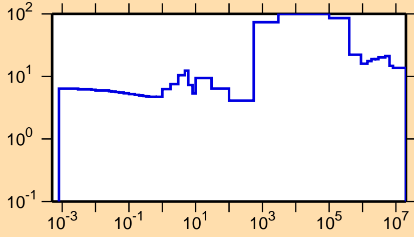
\Delta\sigma/\sigma vs. E for ^{147}\text{Pr}(n,\text{tot.})
