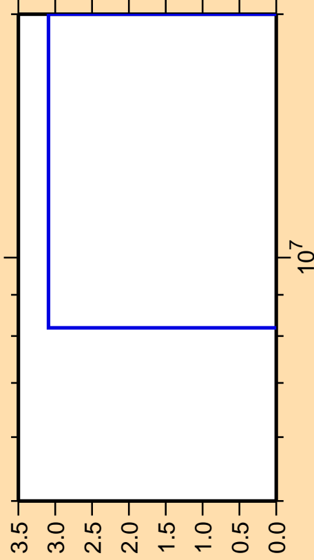
\Delta\sigma/\sigma vs. E for ^{147}\text{Pr}(n,3n\alpha)
