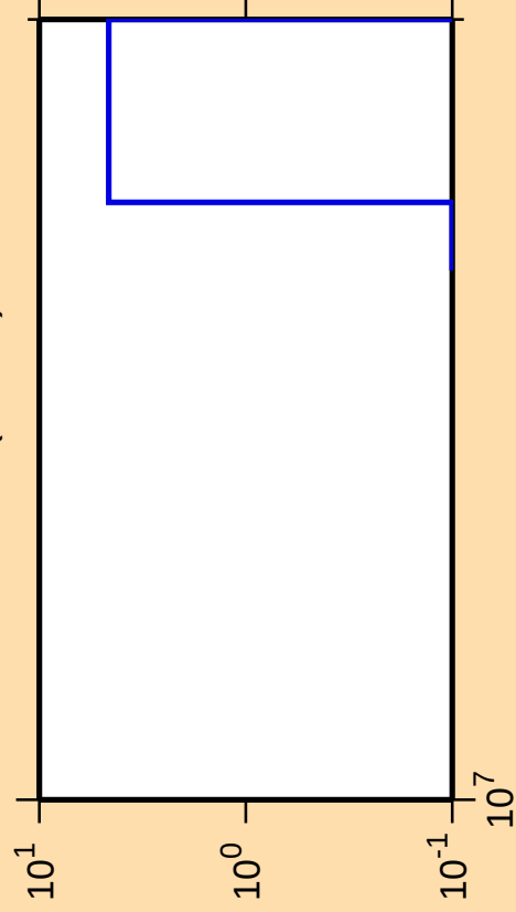
\Delta\sigma/\sigma vs. E for ^{148}\text{Pr}(\text{mt 11})
