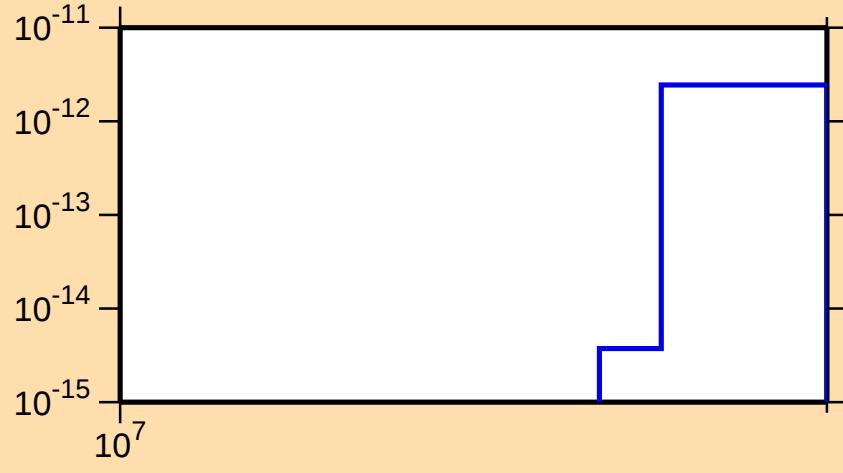
\sigma vs. E for ^{148}\text{Pr}(n,\text{He3})
