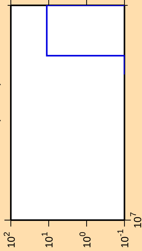
\Delta\sigma/\sigma vs. E for ^{148}\text{Pr}(n,\text{He3})
