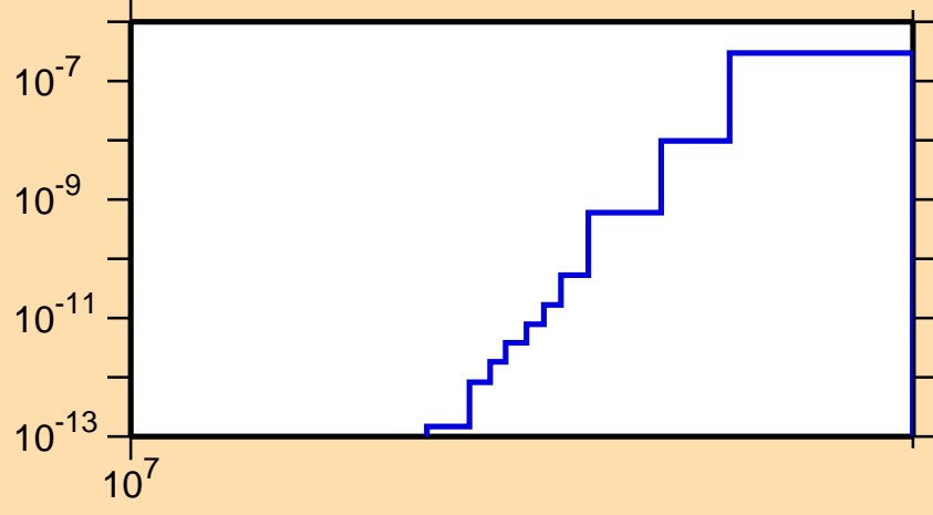
\sigma vs. E for ^{149}\text{Pr}(n,2n\alpha)
