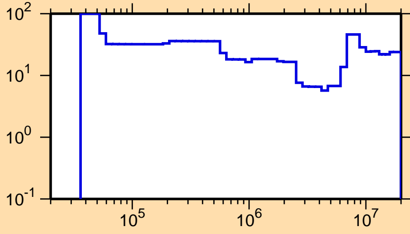
\Delta\sigma/\sigma vs. E for ^{149}\text{Pr}(n,\text{inel.})
