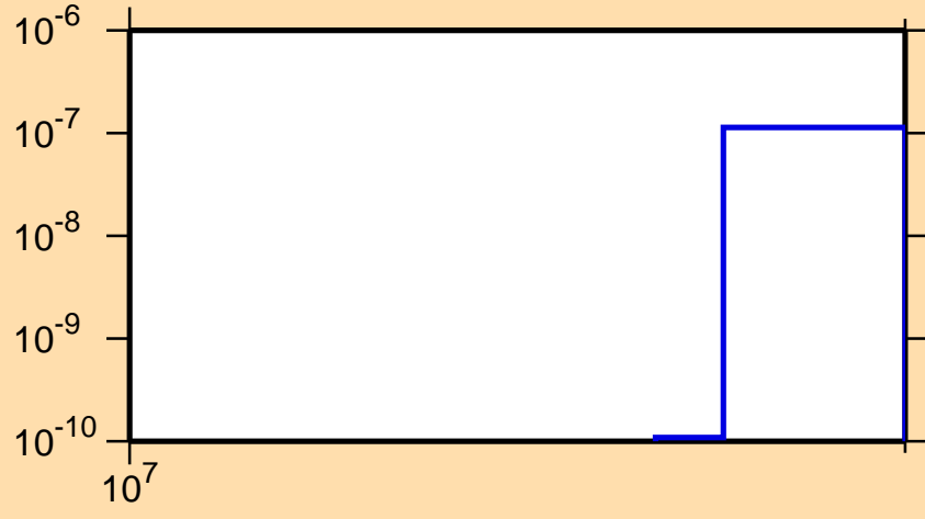
\sigma vs. E for ^{149}\text{Pr}(n,2np)
