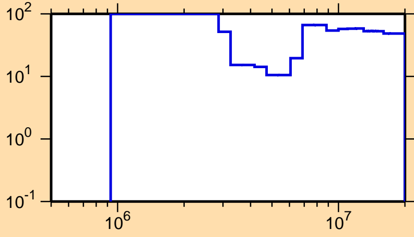
\Delta\sigma/\sigma vs. E for ^{149}\text{Pr}(n,n\text{cont.})
