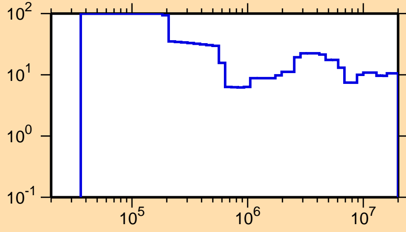
\Delta\sigma/\sigma vs. E for ^{149}\text{Pr}(n,\text{el.})
