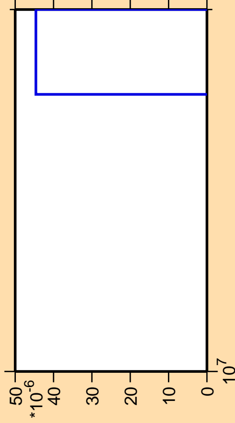
\Delta\sigma/\sigma vs. E for ^{149}\text{Pr}(\text{mt } 42)
