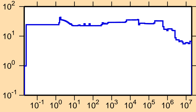
\Delta\sigma/\sigma vs. E for ^{149}\text{Pr}(n,\text{nonel.})
