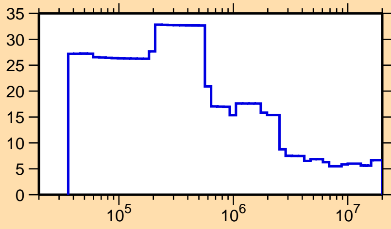
\Delta\sigma/\sigma vs. E for ^{149}\text{Pr}(n,\text{nonel.})
