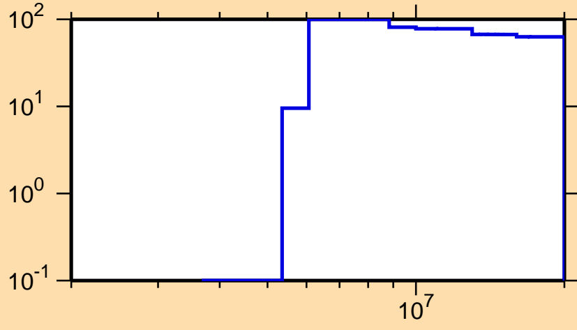
\Delta\sigma/\sigma vs. E for ^{149}\text{Pr}(n,p)
