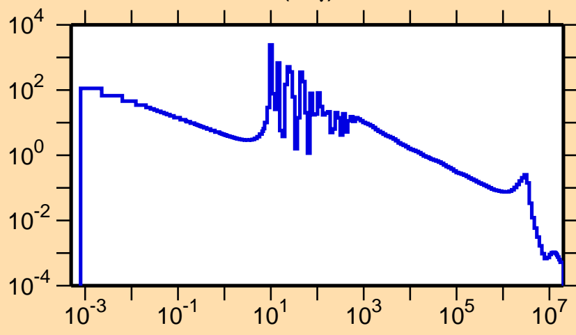
\sigma vs. E for ^{149}\text{Pr}(n,\gamma)
