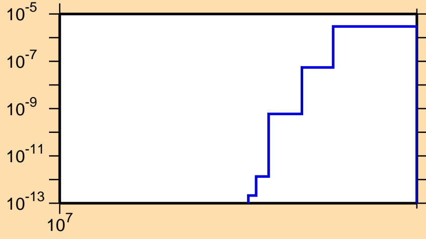
\sigma vs. E for ^{149}\text{Pr}(n,\text{nd})
