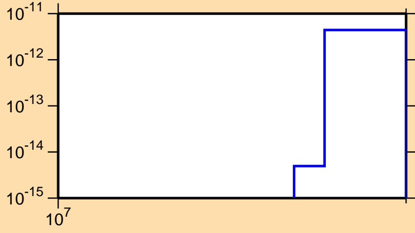
\sigma vs. E for ^{149}\text{Pr}(n,3n\alpha)
