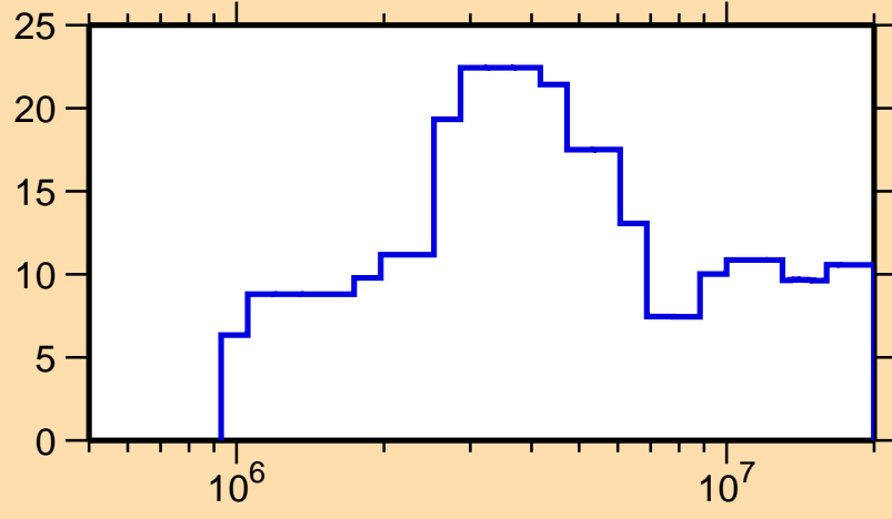
\Delta\sigma/\sigma vs. E for ^{149}\text{Pr}(n, \text{el.})
