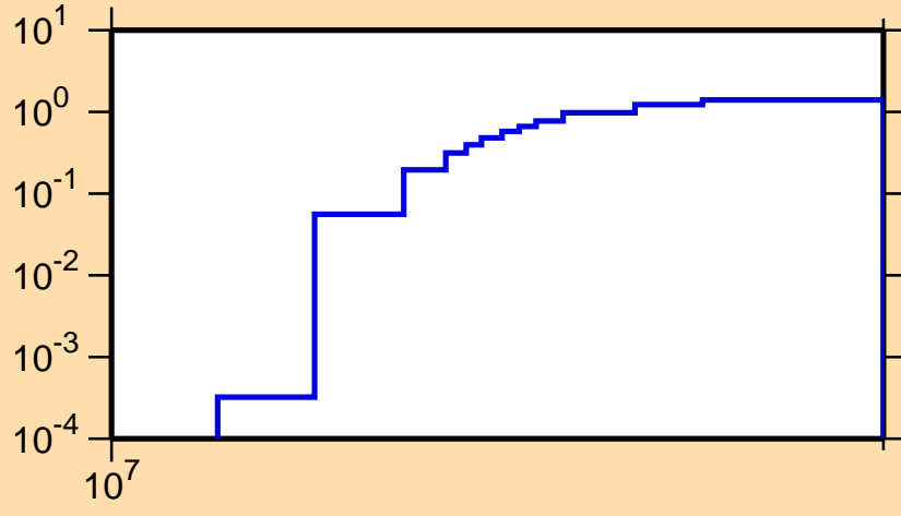
\sigma vs. E for ^{149}\text{Pr}(n,3n)
