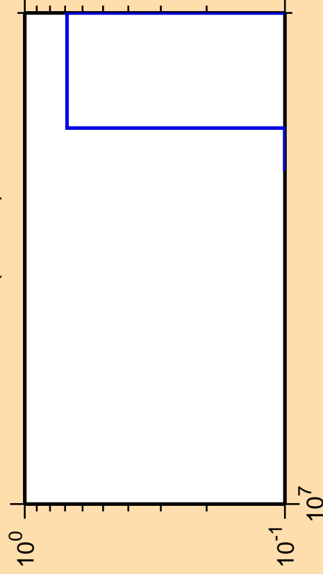
\Delta\sigma/\sigma vs. E for ^{149}\text{Pr}(\text{mt 11})
