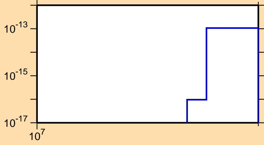
\sigma vs. E for ^{149}\text{Pr}(\text{mt 11})
