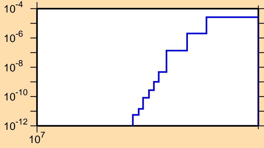
\sigma vs. E for ^{149}\text{Pr}(n,nt)
