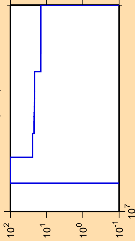
\Delta\sigma/\sigma vs. E for ^{149}\text{Pr}(n,3n)
