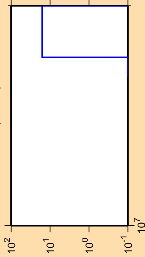
\Delta\sigma/\sigma vs. E for ^{149}\text{Pr}(n,3n\alpha)
