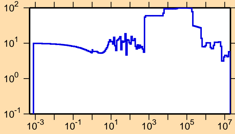
\Delta\sigma/\sigma vs. E for ^{149}\text{Pr}(n,\text{tot.})
