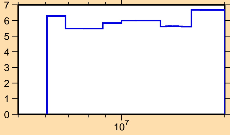
\Delta\sigma/\sigma vs. E for ^{149}\text{Pr}(n,\text{nonel.})
