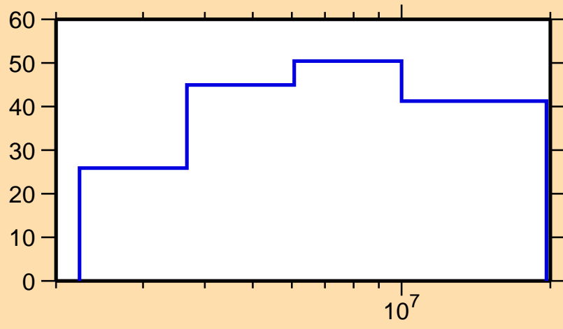
\Delta\sigma/\sigma vs. E for ^{149}\text{Pr}(n,n_1)
