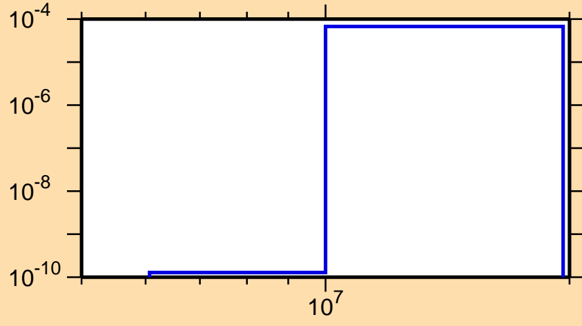
\sigma vs. E for ^{149}\text{Pr}(n,n\alpha)
