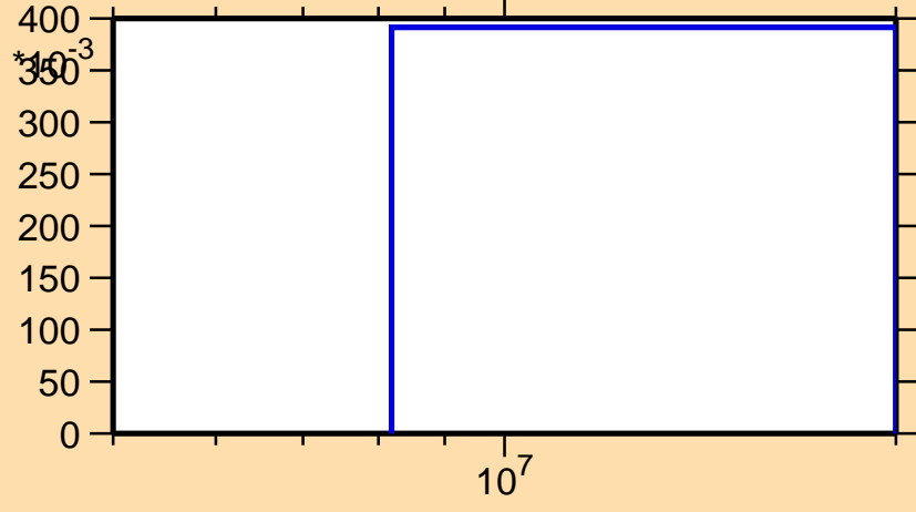
\sigma vs. E for ^{149}\text{Pr}(n,3n)
