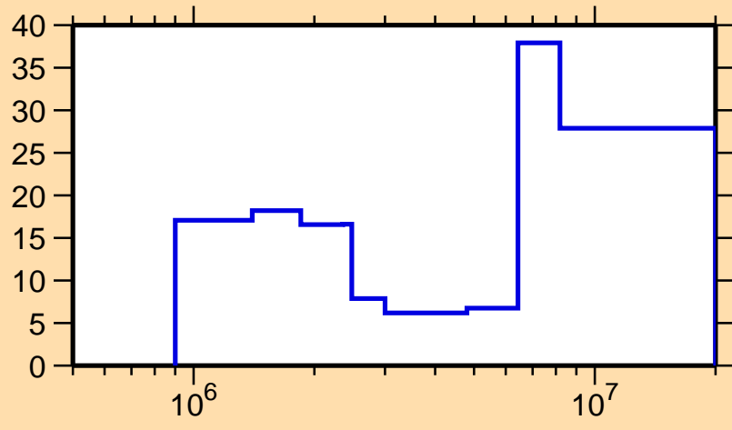
\Delta\sigma/\sigma vs. E for ^{149}\text{Pr}(n,incl.)
