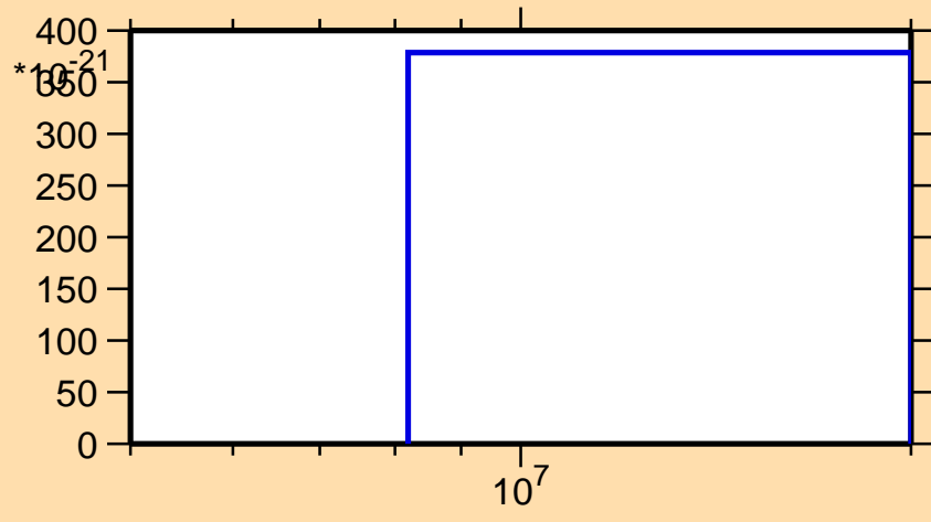
\sigma vs. E for ^{149}\text{Pr}(\text{mt } 42)
