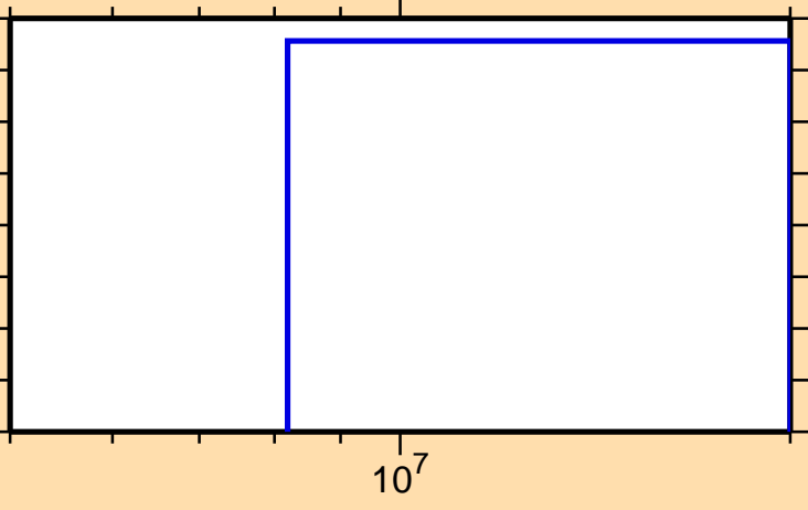
\sigma vs. E for ^{149}\text{Pr}(n,3n\alpha)
