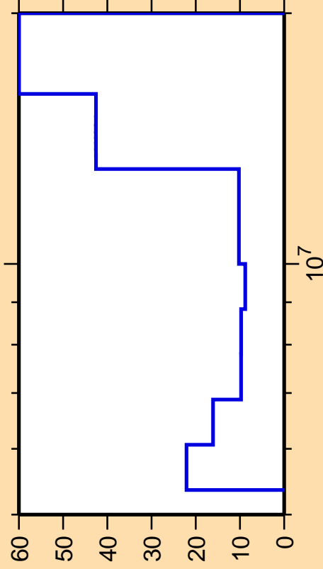
\Delta\sigma/\sigma vs. E for ^{150}\text{Pr}(n,2n)
