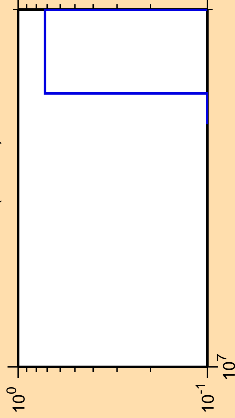
\Delta\sigma/\sigma vs. E for ^{150}\text{Pr}(n,3n\alpha)
