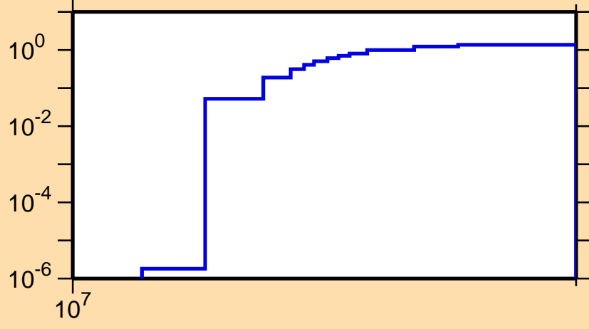
\sigma vs. E for ^{150}\text{Pr}(n,3n)
