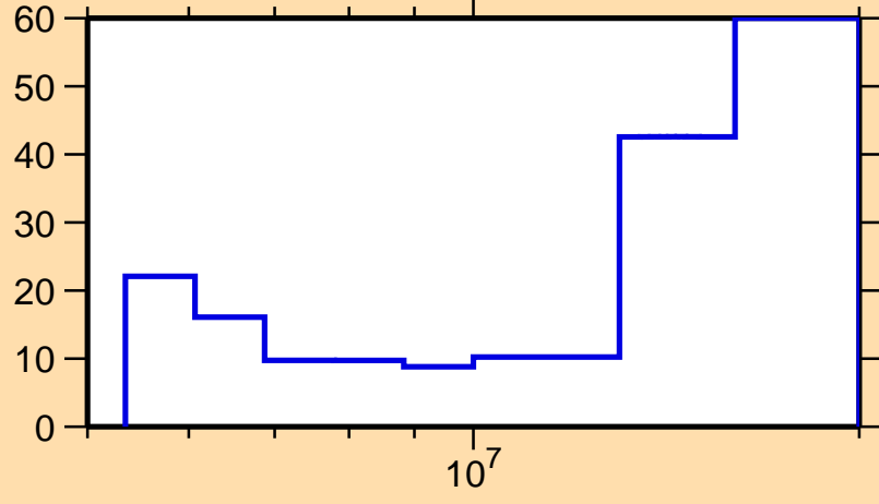
\Delta\sigma/\sigma vs. E for ^{150}\text{Pr}(n,2n)
