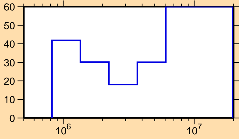
\Delta\sigma/\sigma vs. E for ^{150}\text{Pr}(n,n\text{cont.})
