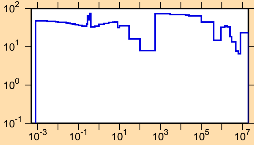
\Delta\sigma/\sigma vs. E for ^{150}\text{Pr}(n,\text{tot.})
