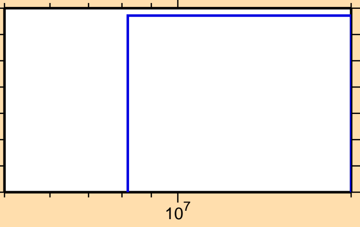
\sigma vs. E for ^{150}\text{Pr}(n,2np)
