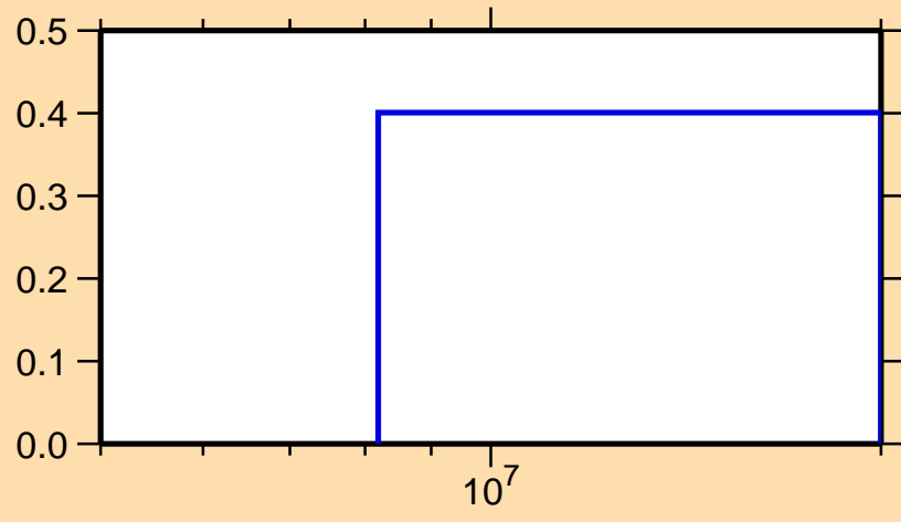
\sigma vs. E for ^{150}\text{Pr}(n,3n)
