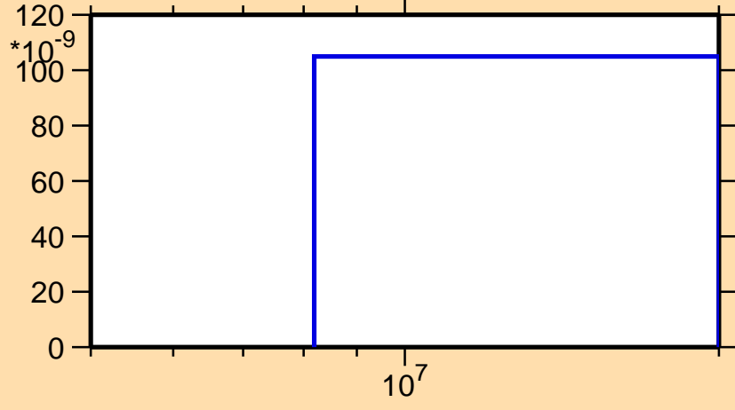
\sigma vs. E for ^{150}\text{Pr}(n,nt)
