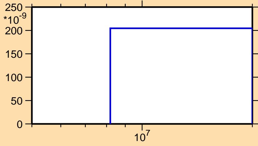
\sigma vs. E for ^{150}\text{Pr}(n,\text{nd})
