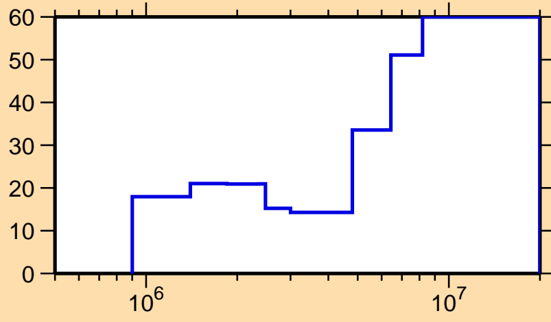
\Delta\sigma/\sigma vs. E for ^{150}\text{Pr}(n,\text{inel.})
