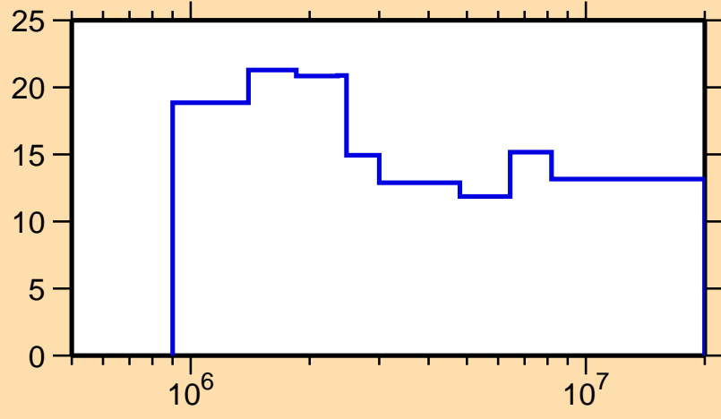
\Delta\sigma/\sigma vs. E for ^{150}\text{Pr}(n,\text{nonel.})
