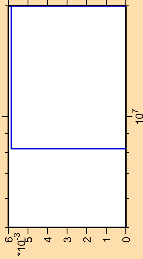
\Delta\sigma/\sigma vs. E for ^{150}\text{Pr}(n,3n\alpha)
