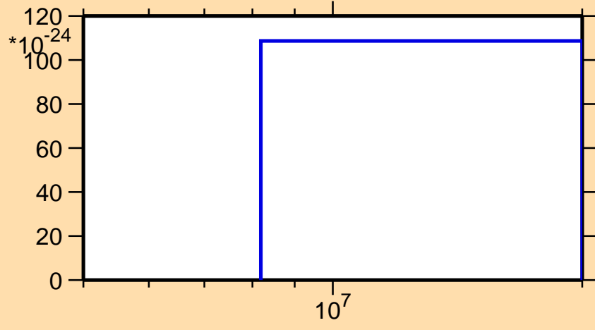
\sigma vs. E for ^{150}\text{Pr}(\text{mt } 42)
