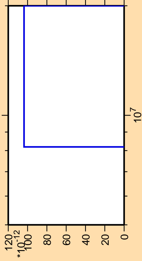
\Delta\sigma/\sigma vs. E for ^{150}\text{Pr}(\text{mt } 42)
