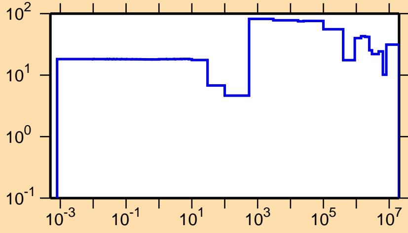
\Delta\sigma/\sigma vs. E for ^{150}\text{Pr}(n,\text{el.})
