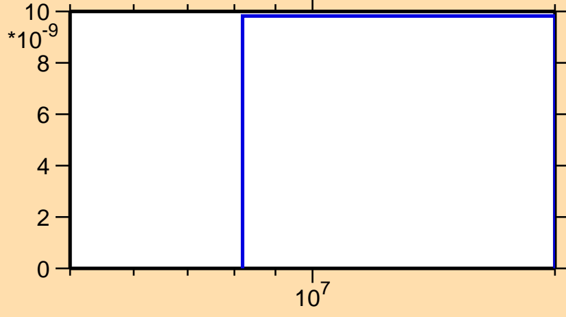
\sigma vs. E for ^{150}\text{Pr}(n,2n\alpha)
