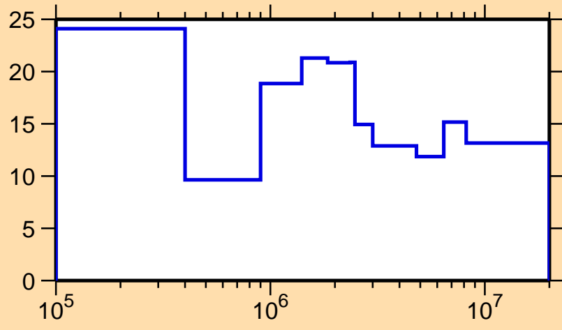
\Delta\sigma/\sigma vs. E for ^{150}\text{Pr}(n,\text{nonel.})
