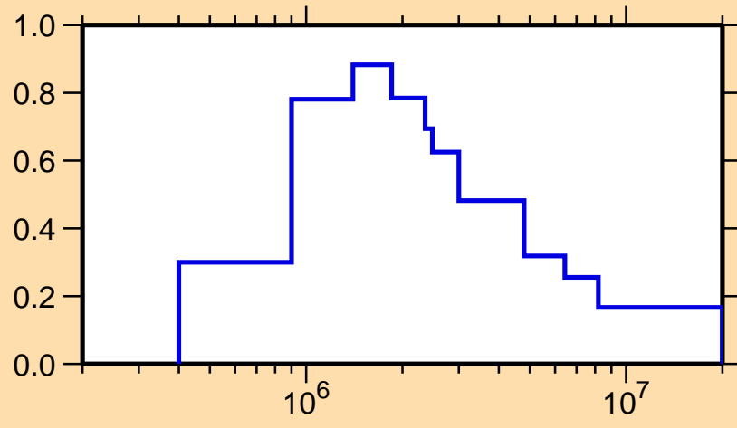
\sigma vs. E for ^{150}\text{Pr}(n,n_3)
