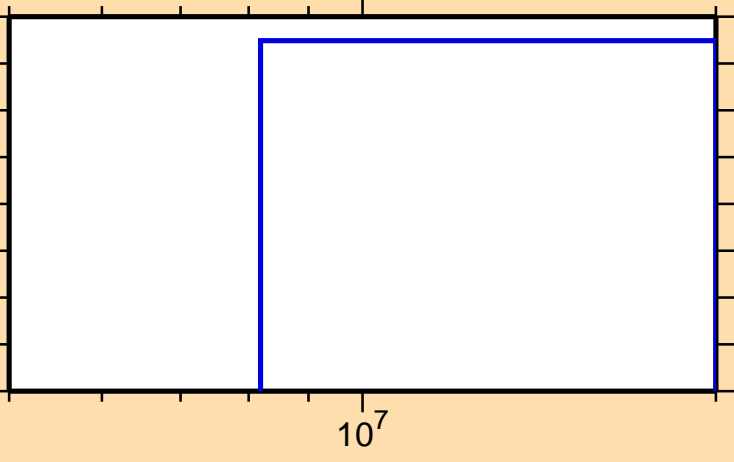
\sigma vs. E for ^{150}\text{Pr}(n,n\alpha)
