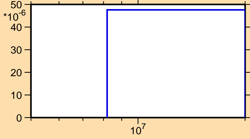
\sigma vs. E for ^{150}\text{Pr}(n,np)
