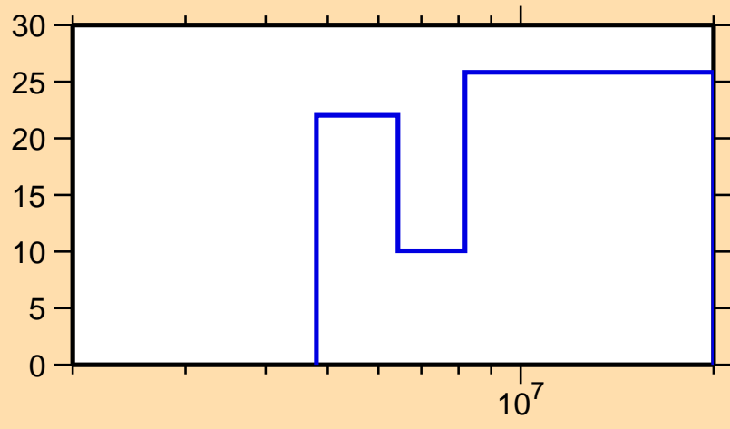
\Delta\sigma/\sigma vs. E for ^{150}\text{Pr}(n,2n)
