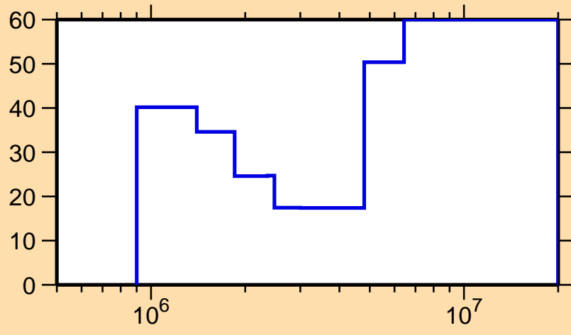
\Delta\sigma/\sigma vs. E for ^{150}\text{Pr}(n,n\text{cont.})
