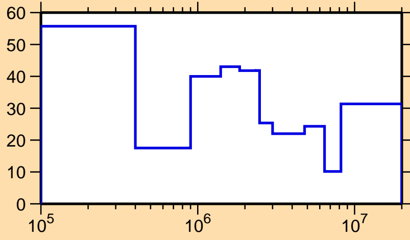
\Delta\sigma/\sigma vs. E for ^{150}\text{Pr}(n,\text{el.})
