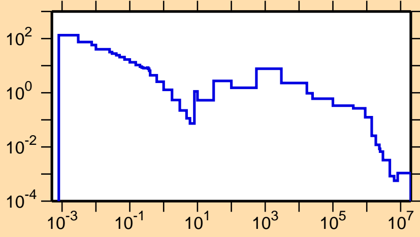
\sigma vs. E for ^{150}\text{Pr}(n,\gamma)
