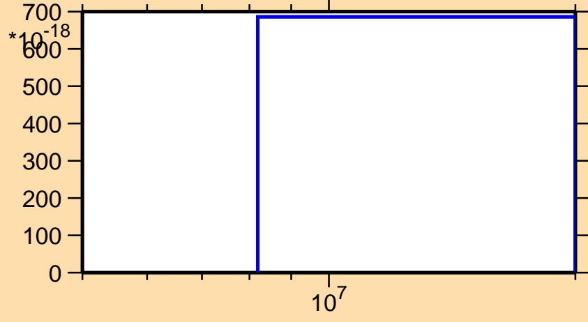
\sigma vs. E for ^{150}\text{Pr}(n,3n\alpha)
