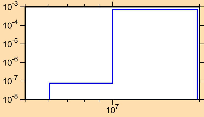
\sigma vs. E for ^{151}\text{Pr}(n,p)
