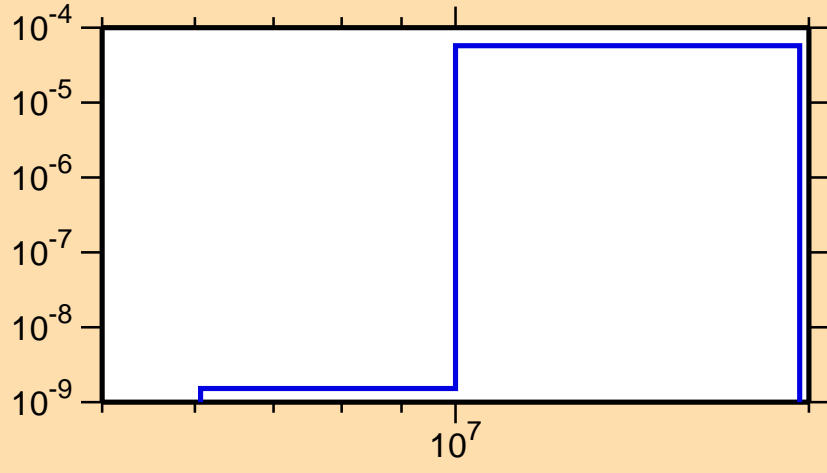
\sigma vs. E for ^{151}\text{Pr}(n,\alpha)
