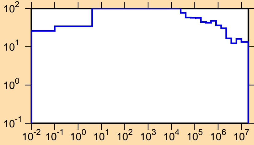
\Delta\sigma/\sigma vs. E for ^{151}\text{Pr}(n,\text{nonel.})
