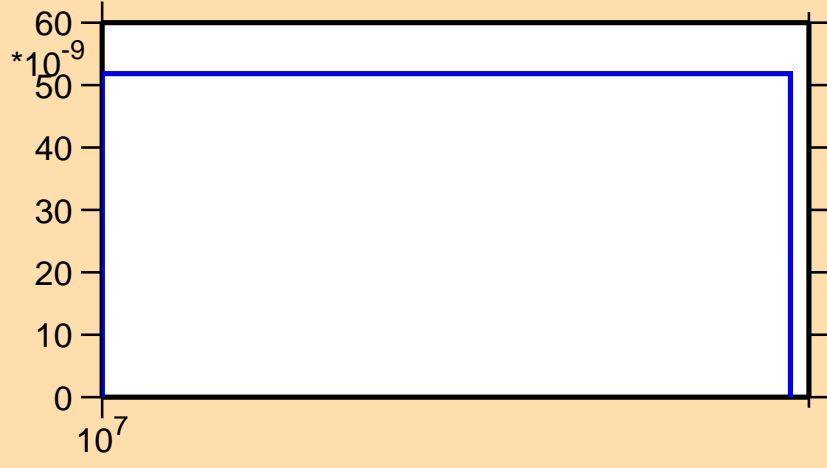
\sigma vs. E for ^{151}\text{Pr}(n,nt)
