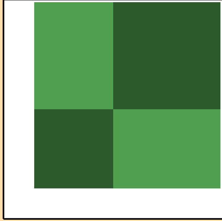
\sigma vs. E for ^{151}\text{Pr}(n,2n)
