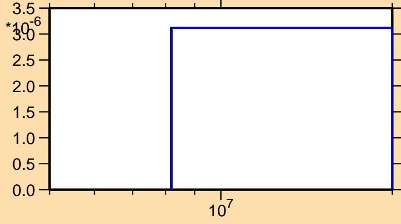
\sigma vs. E for ^{151}\text{Pr}(n,n\alpha)
