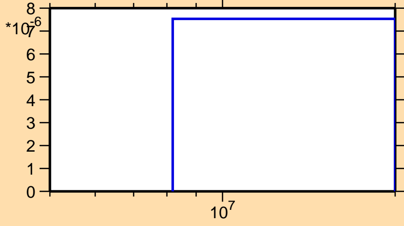
\sigma vs. E for ^{151}\text{Pr}(n,t)
