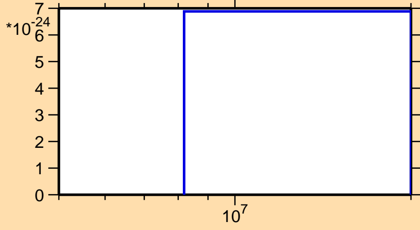
\sigma vs. E for ^{151}\text{Pr}(\text{mt } 42)
