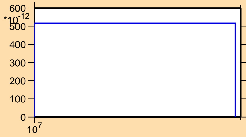
\sigma vs. E for ^{154}\text{Pr}(n,2np)
