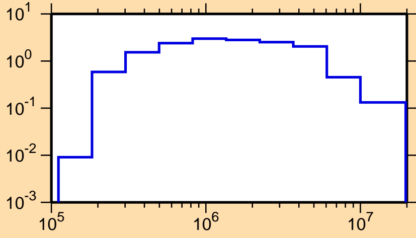
\sigma vs. E for ^{154}\text{Pr}(n,n\text{cont.})
