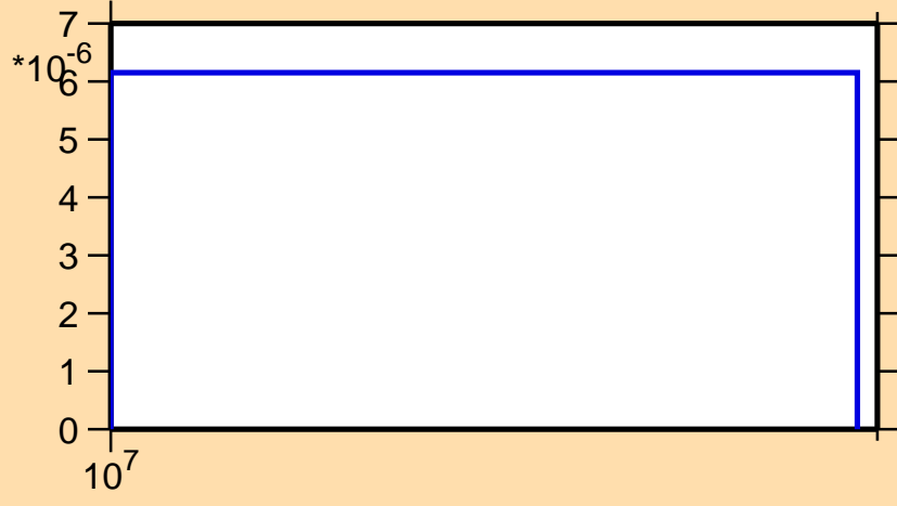
\sigma vs. E for ^{154}\text{Pr}(n,np)
