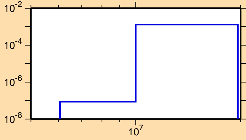
\sigma vs. E for ^{154}\text{Pr}(n,p)
