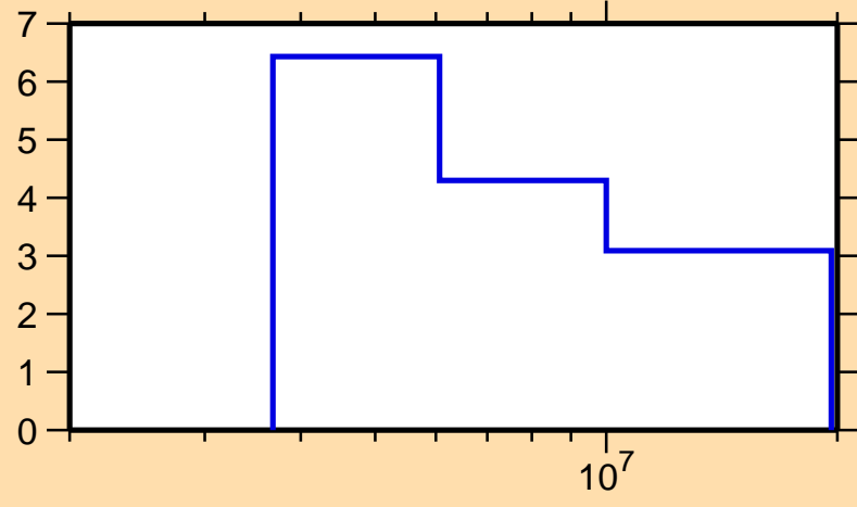
\Delta\sigma/\sigma vs. E for ^{154}\text{Pr}(n,\text{tot.})
