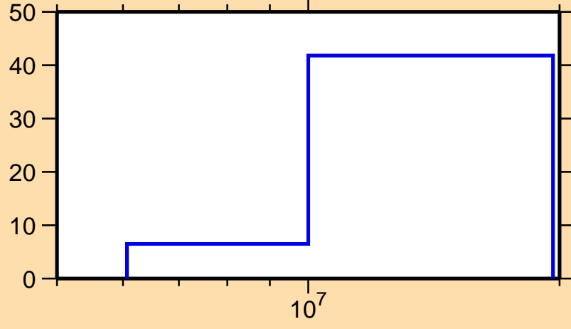
\Delta\sigma/\sigma vs. E for ^{154}\text{Pr}(n,2n)
