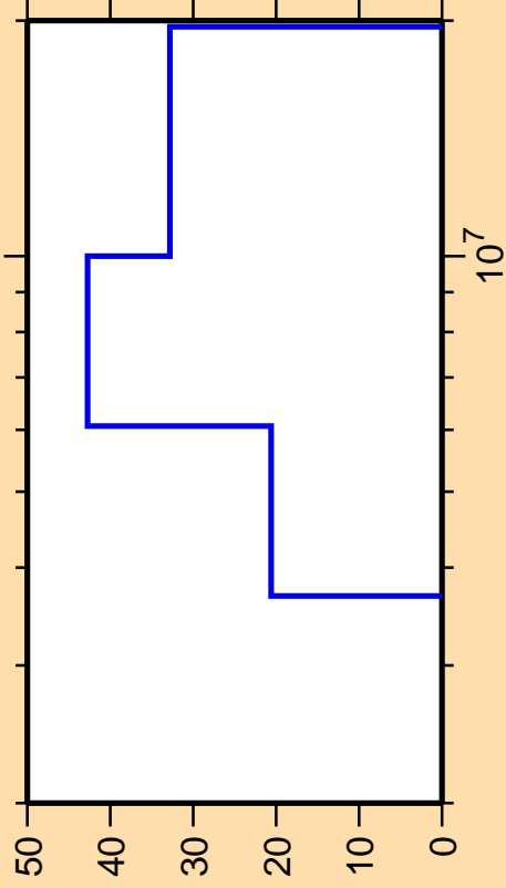
\Delta\sigma/\sigma vs. E for ^{154}\text{Pr}(n,n\text{cont.})
