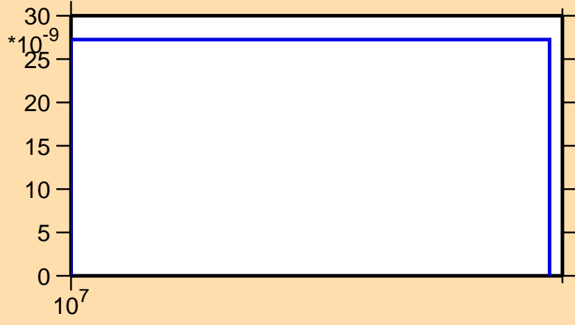
\sigma vs. E for ^{154}\text{Pr}(n,nt)
