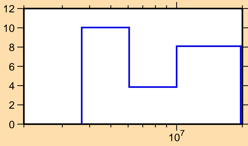
\Delta\sigma/\sigma vs. E for ^{154}\text{Pr}(n,\text{el.})
