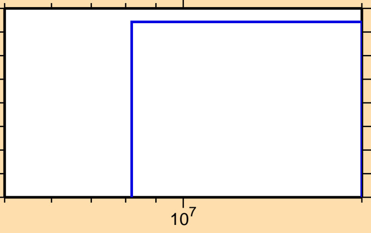
\sigma vs. E for ^{154}\text{Pr}(n,2n\alpha)
