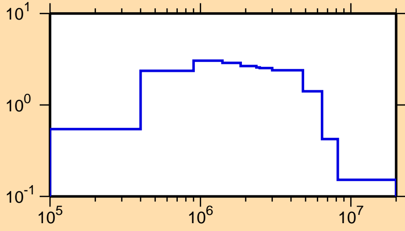
\sigma vs. E for ^{154}\text{Pr}(n,\text{inel.})
