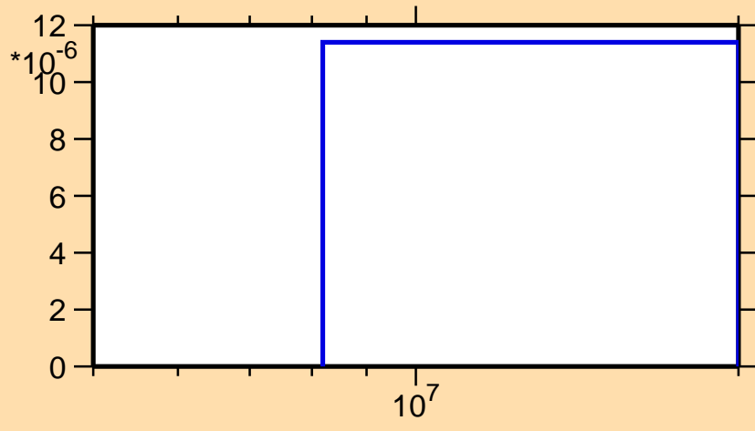
\sigma vs. E for ^{154}\text{Pr}(n,d)
