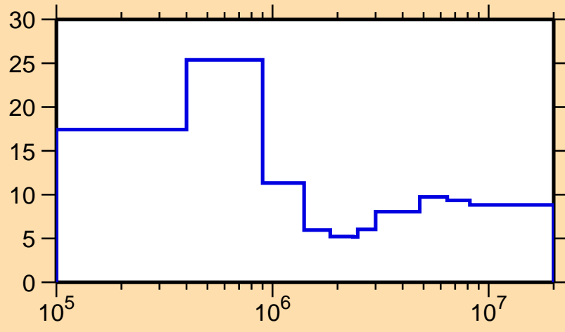
\Delta\sigma/\sigma vs. E for ^{154}\text{Pr}(n,n\text{onel.})
