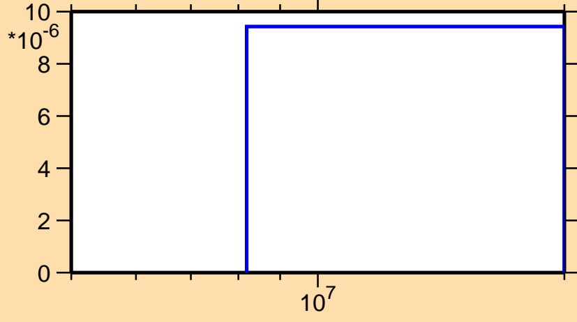
\sigma vs. E for ^{154}\text{Pr}(n,t)
