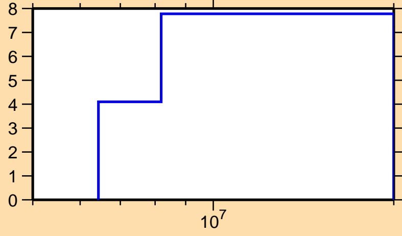
\Delta\sigma/\sigma vs. E for ^{154}\text{Pr}(n,\text{el.})
