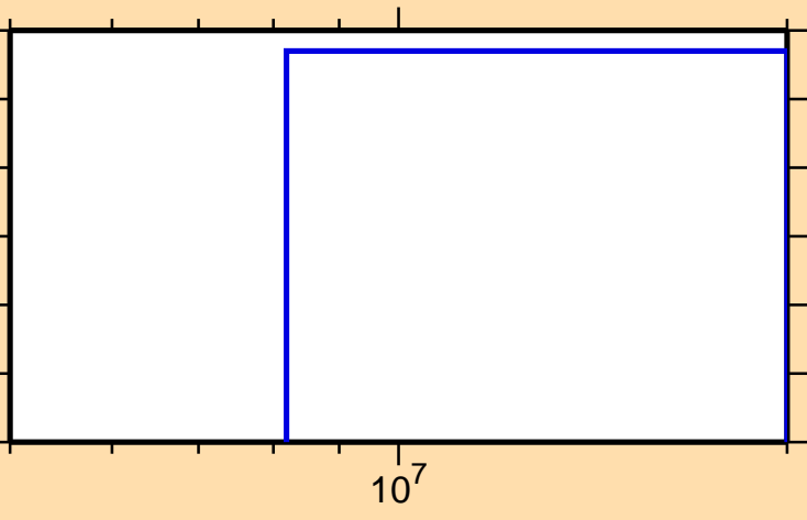
\sigma vs. E for ^{154}\text{Pr}(n,d)
