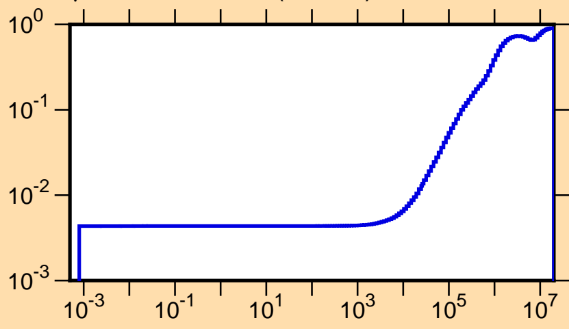
\mu vs. E for ^{155}\text{Pr}(\text{mt251})
