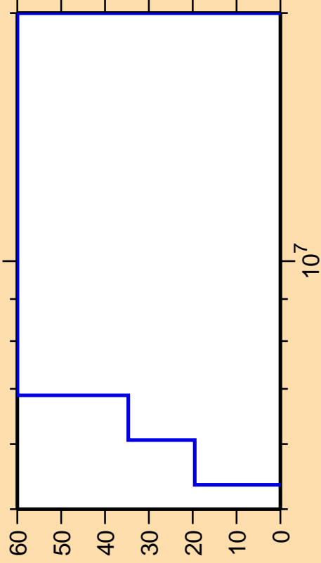
\Delta\sigma/\sigma vs. E for ^{155}\text{Pr}(n,n\text{cont.})
