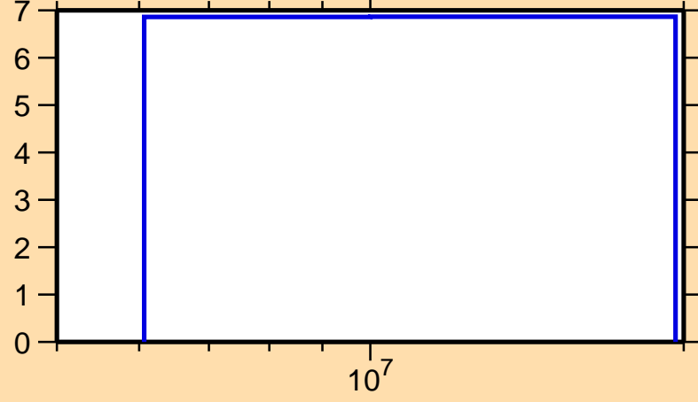
\Delta\sigma/\sigma vs. E for ^{155}\text{Pr}(n,\text{tot.})
