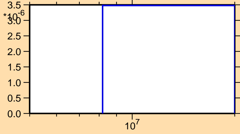
\sigma vs. E for ^{155}\text{Pr}(n,\alpha)
