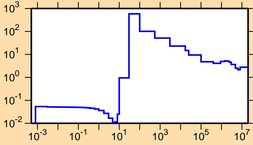
\sigma vs. E for ^{155}\text{Pr}(n,\text{el.})
