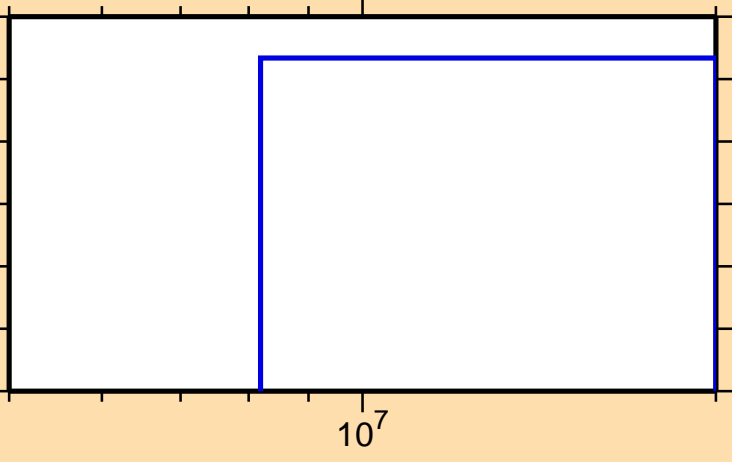
\sigma vs. E for ^{155}\text{Pr}(n,p)
