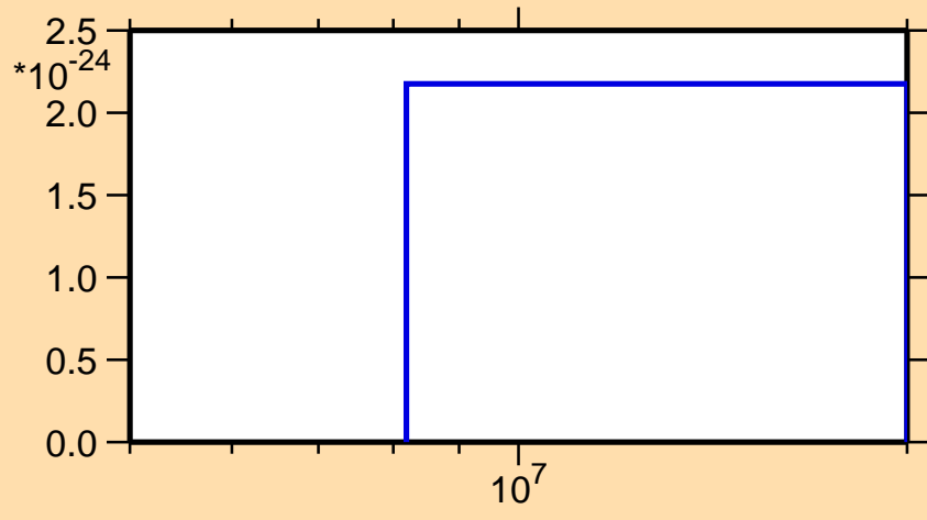
\sigma vs. E for ^{155}\text{Pr}(\text{mt } 42)
