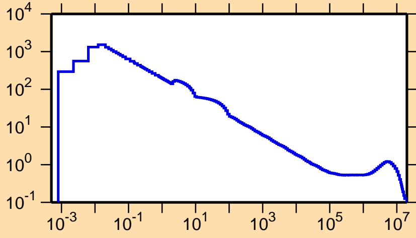
\sigma vs. E for ^{175}\text{Pt}(n,p)
