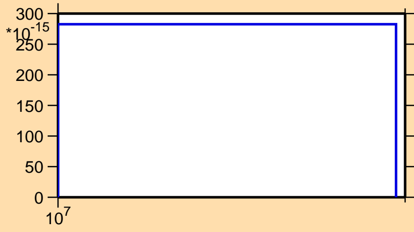
\sigma vs. E for ^{175}\text{Pt}(n,nt)
