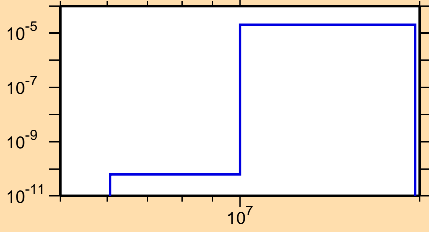
\sigma vs. E for ^{175}\text{Pt}(n,\text{pd})
