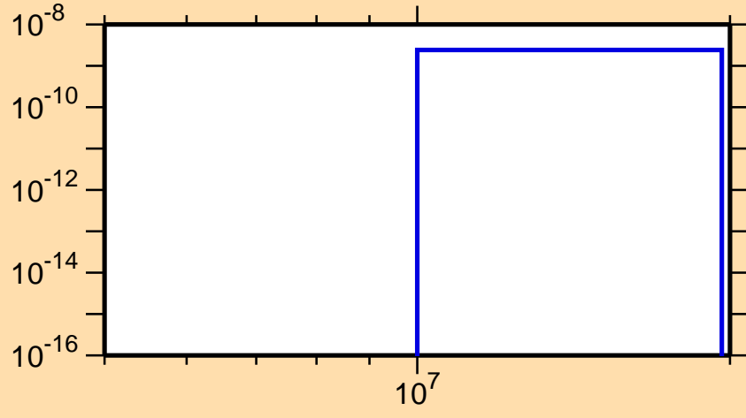
\sigma vs. E for ^{175}\text{Pt}(\text{mt } 34)
