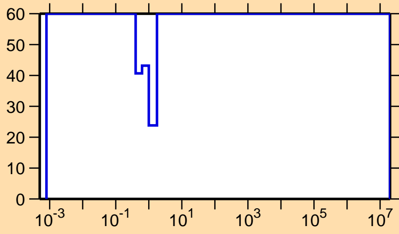
\Delta\sigma/\sigma vs. E for ^{175}\text{Pt}(n,\gamma)
