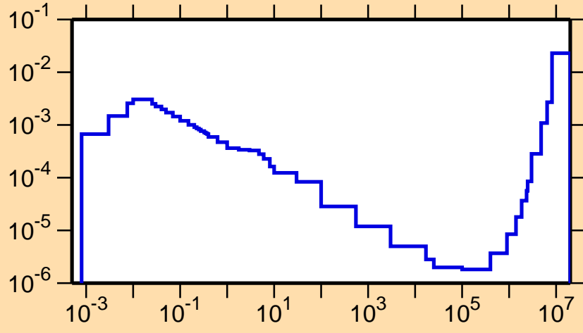
\sigma vs. E for ^{175}\text{Pt}(n,p\alpha)
