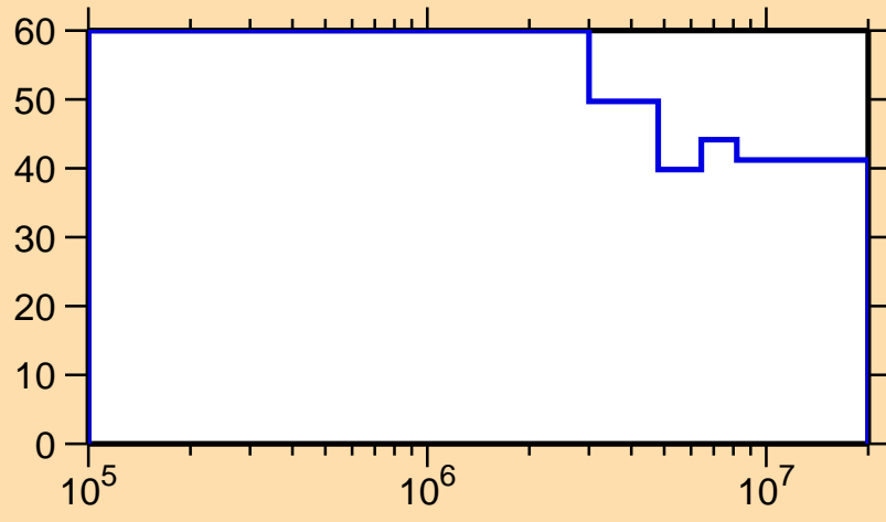
\Delta\sigma/\sigma vs. E for ^{175}\text{Pt}(n,\text{inel.})
