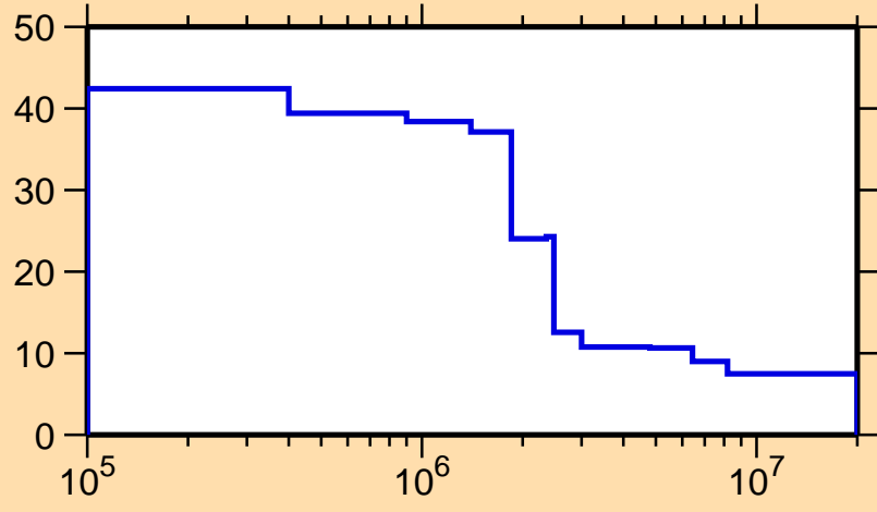
\Delta\sigma/\sigma vs. E for ^{175}\text{Pt}(n,\text{nonel.})
