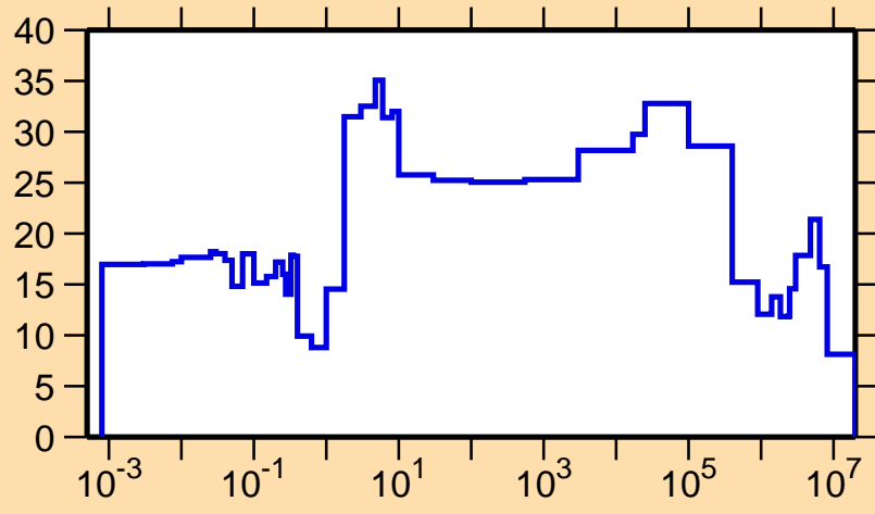
\Delta\sigma/\sigma vs. E for ^{175}\text{Pt}(n,\text{el.})
