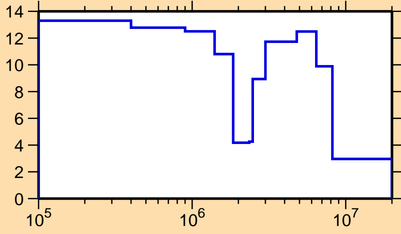
\Delta\sigma/\sigma vs. E for ^{175}\text{Pt}(n,\text{tot.})
