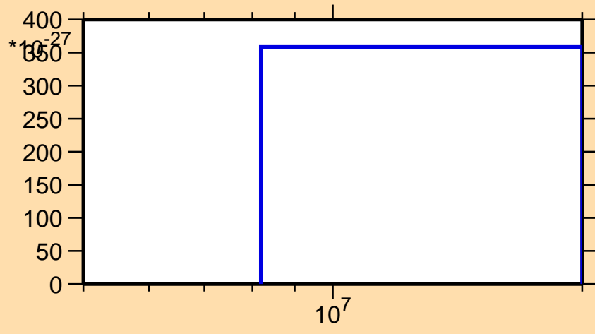
\sigma vs. E for ^{175}\text{Pt}(\text{mt } 11)
