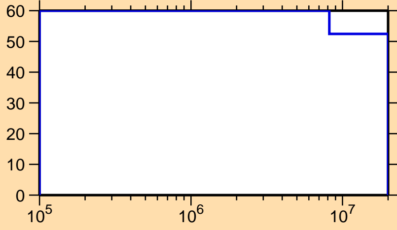
\Delta\sigma/\sigma vs. E for ^{175}\text{Pt}(n,n_1)
