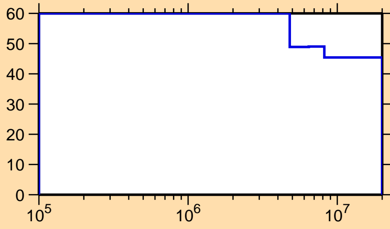
\Delta\sigma/\sigma vs. E for ^{175}\text{Pt}(n,n\text{cont.})
