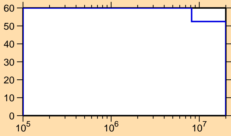
\Delta\sigma/\sigma vs. E for ^{175}\text{Pt}(n,n_1)
