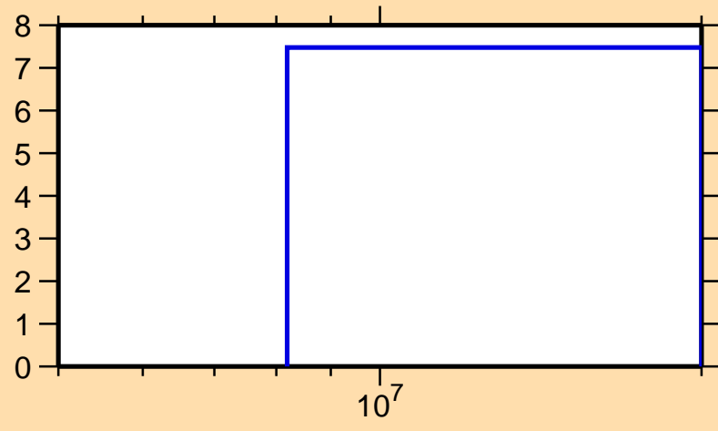
\Delta\sigma/\sigma vs. E for ^{175}\text{Pt}(n,\text{nonel.})
