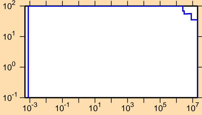
\Delta\sigma/\sigma vs. E for ^{175}\text{Pt}(n,p)
