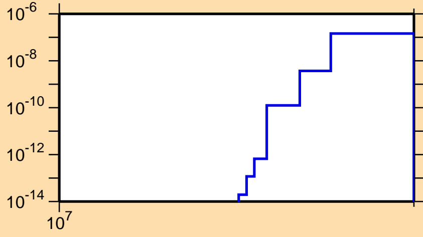
\sigma vs. E for ^{176}\text{Pt}(n,\text{nd})
