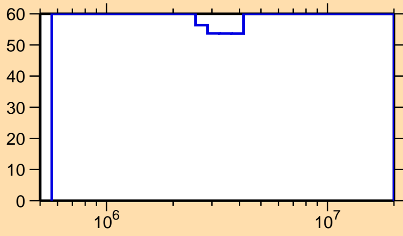
\Delta\sigma/\sigma vs. E for ^{176}\text{Pt}(n, \text{inel.})
