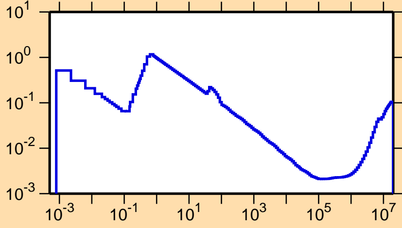
\sigma vs. E for ^{176}\text{Pt}(n,\alpha)
