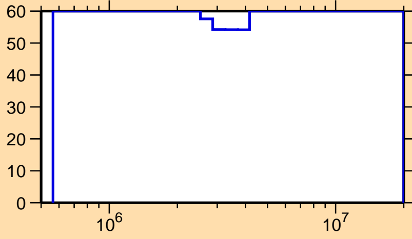
\Delta\sigma/\sigma vs. E for ^{176}\text{Pt}(n,n_1)
