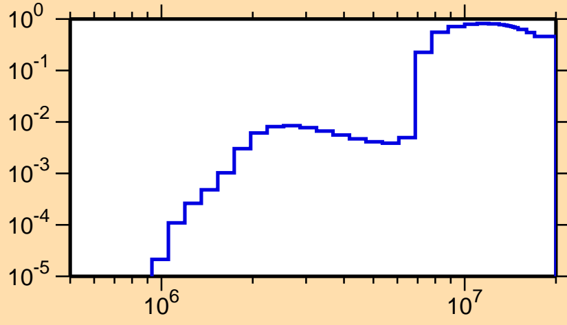
\sigma vs. E for ^{176}\text{Pt}(n,n\text{cont.})
