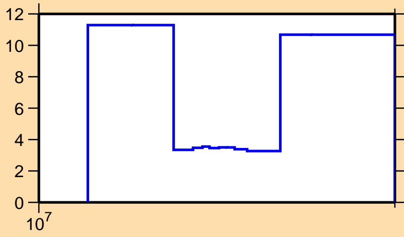
\Delta\sigma/\sigma vs. E for ^{176}\text{Pt}(n,\text{tot.})
