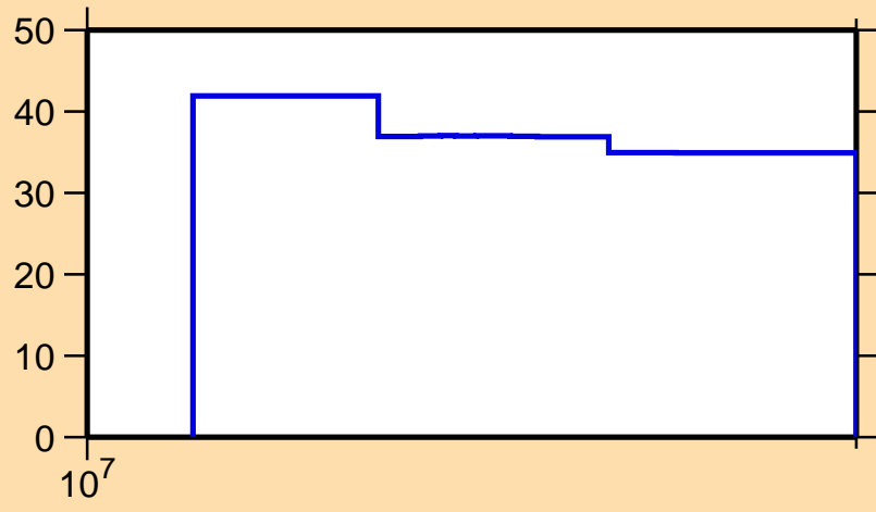
\Delta\sigma/\sigma vs. E for ^{176}\text{Pt}(n,\text{nonel.})
