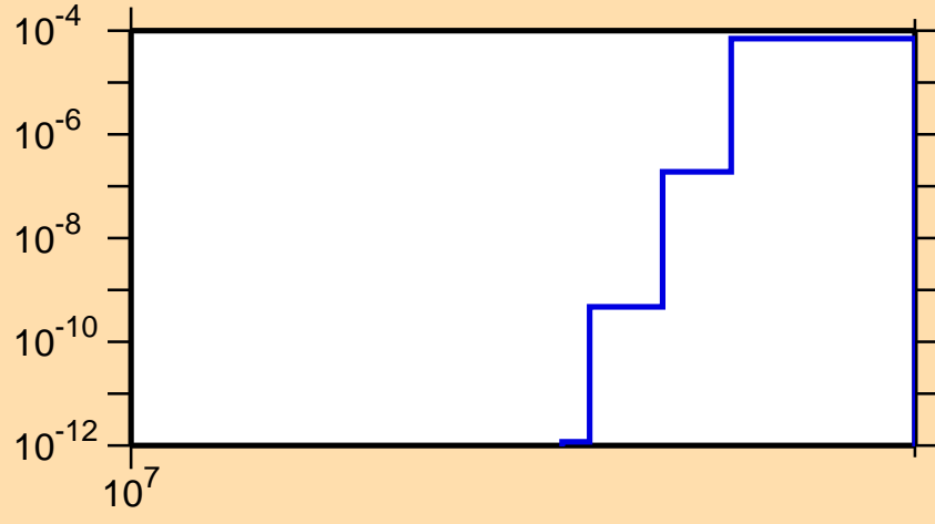
\sigma vs. E for ^{176}\text{Pt}(n,2np)
