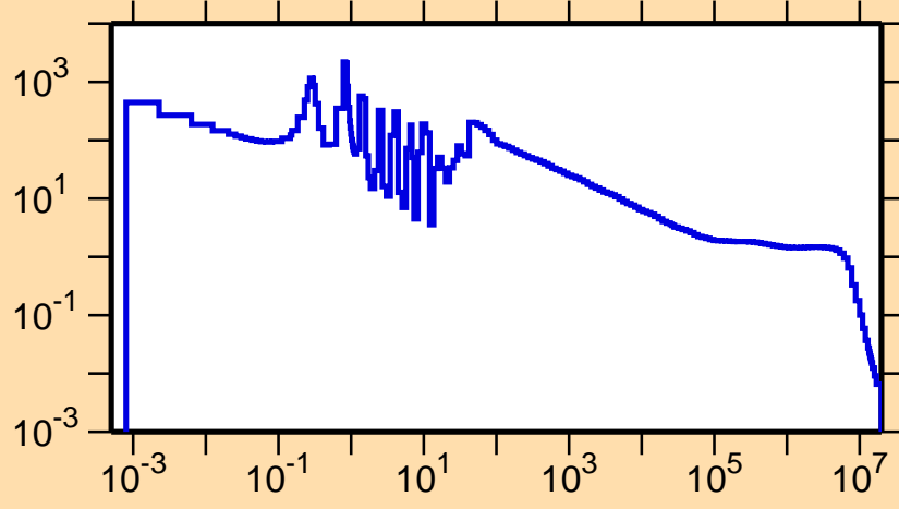
\sigma vs. E for ^{176}\text{Pt}(n,\gamma)
