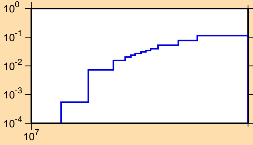
\sigma vs. E for ^{176}\text{Pt}(n,2n)
