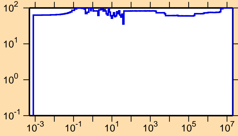
\Delta\sigma/\sigma vs. E for ^{176}\text{Pt}(n,\gamma)
