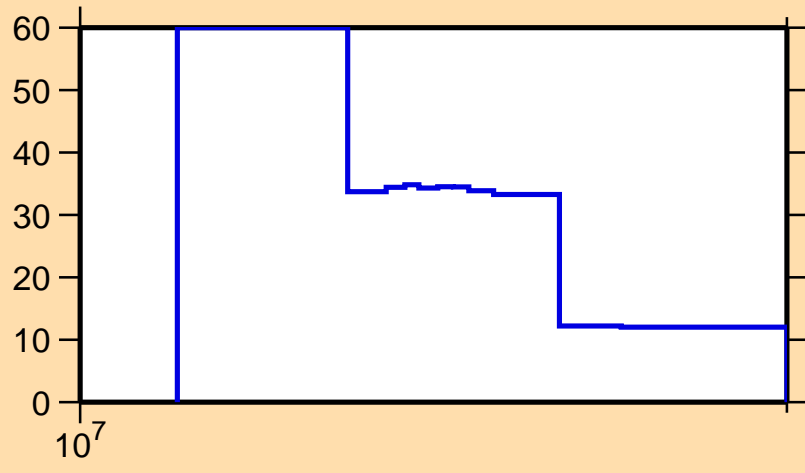
\Delta\sigma/\sigma vs. E for ^{176}\text{Pt}(n,\text{el.})
