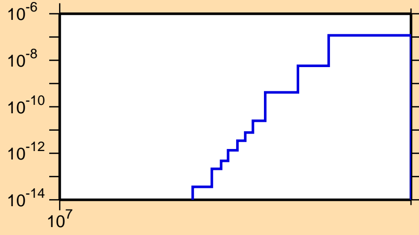
\sigma vs. E for ^{176}\text{Pt}(n,\text{pt})
