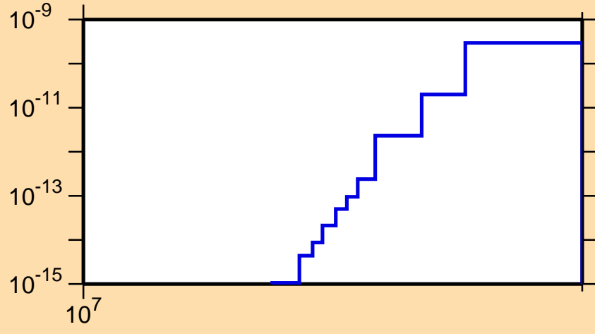
\sigma vs. E for ^{176}\text{Pt}(\text{mt } 34)
