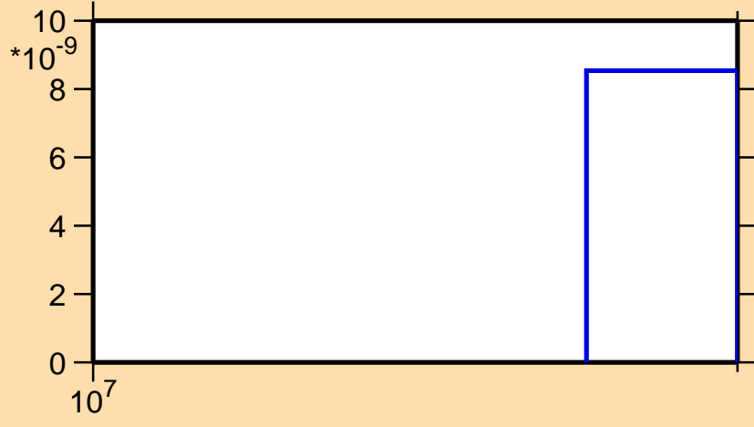
\sigma vs. E for ^{176}\text{Pt}(n,3n)
