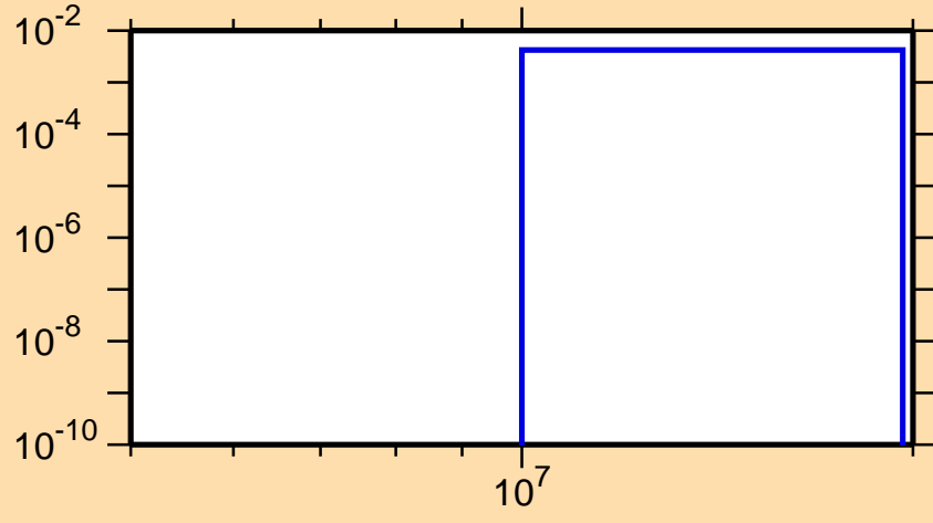
\sigma vs. E for ^{176}\text{Pt}(n,2n\alpha)
