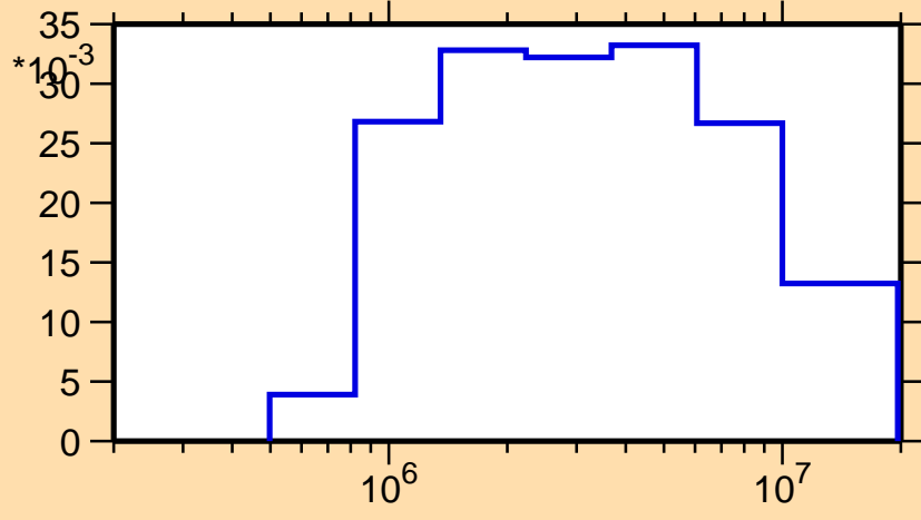
\sigma vs. E for ^{176}\text{Pt}(n,n_3)
