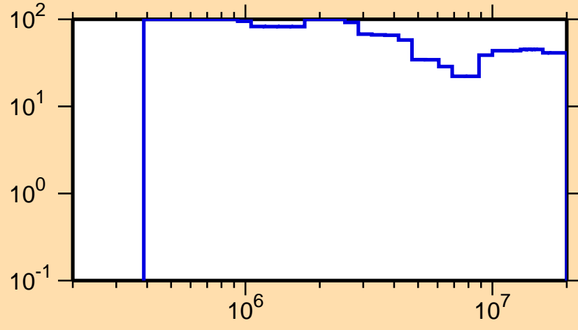
\Delta\sigma/\sigma vs. E for ^{177}\text{Pt}(n,n\text{cont.})
