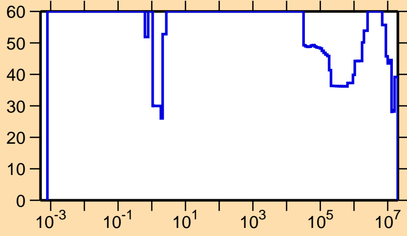
\Delta\sigma/\sigma vs. E for ^{177}\text{Pt}(n,\gamma)
