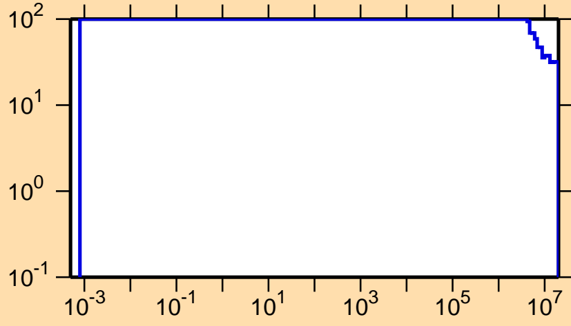
\Delta\sigma/\sigma vs. E for ^{177}\text{Pt}(n,p)
