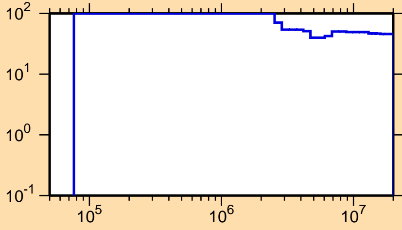
\Delta\sigma/\sigma vs. E for ^{177}\text{Pt}(n,n_1)
