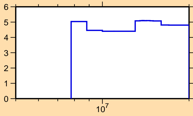
\Delta\sigma/\sigma vs. E for ^{177}\text{Pt}(n,\text{nonel.})
