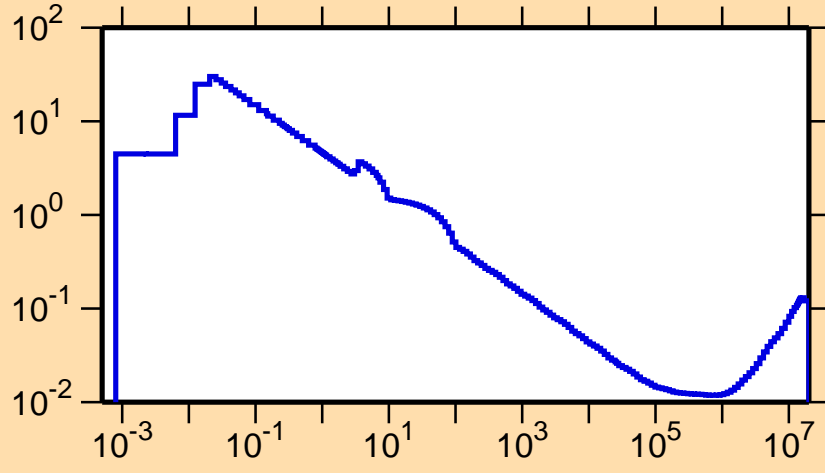
\sigma vs. E for ^{177}\text{Pt}(n,\alpha)
