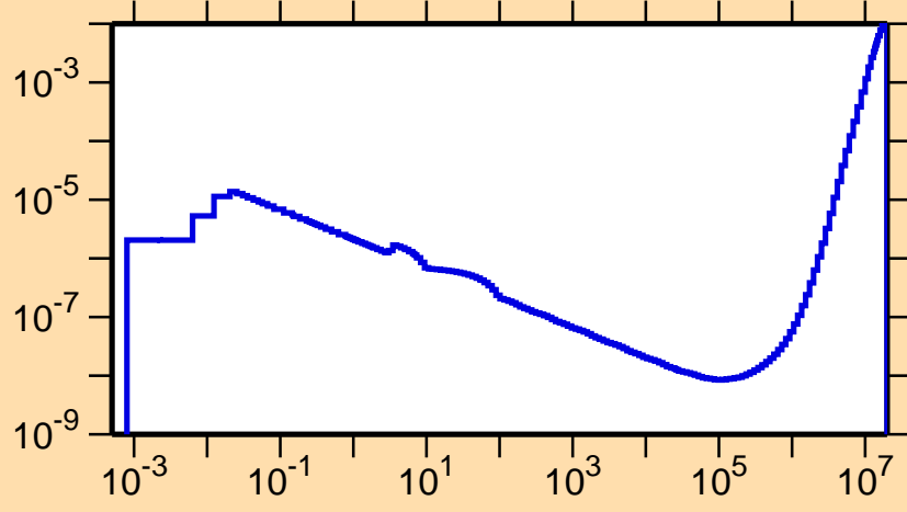
\sigma vs. E for ^{177}\text{Pt}(n,p\alpha)
