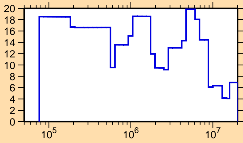
\Delta\sigma/\sigma vs. E for ^{177}\text{Pt}(n,\text{el.})
