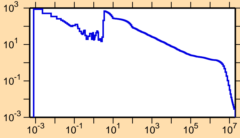
\sigma vs. E for ^{177}\text{Pt}(n,\gamma)
