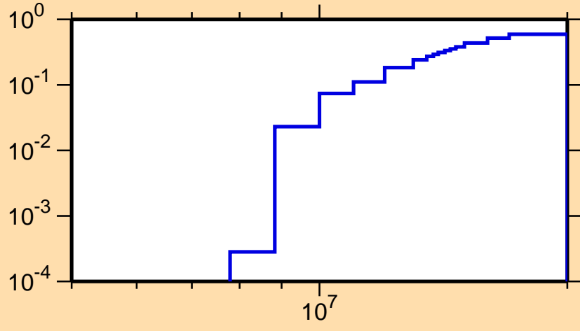
\sigma vs. E for ^{177}\text{Pt}(n,2n)
