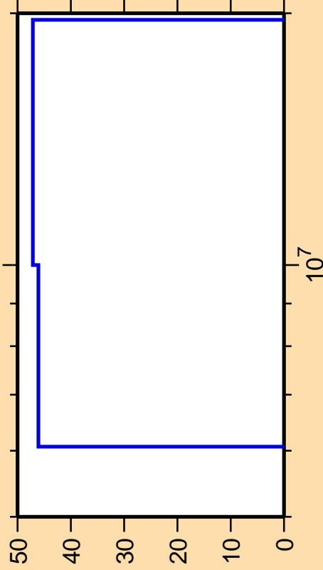
\Delta\sigma/\sigma vs. E for ^{177}\text{Pt}(n,n_1)
