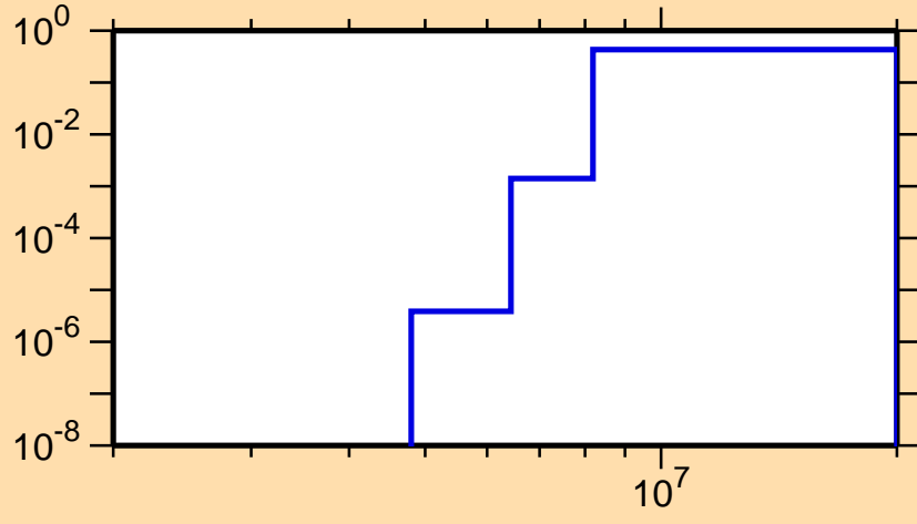
\sigma vs. E for ^{177}\text{Pt}(n,np)
