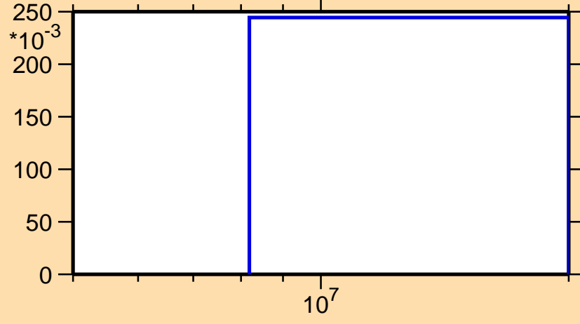
\sigma vs. E for ^{177}\text{Pt}(n,2n)
