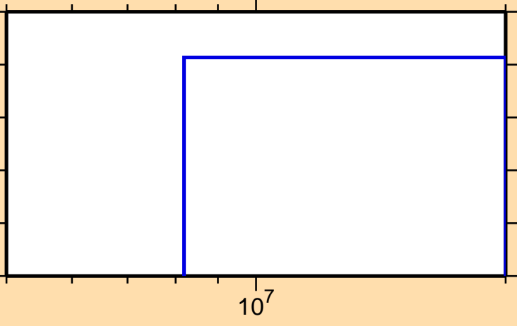
\sigma vs. E for ^{177}\text{Pt}(\text{mt117})
