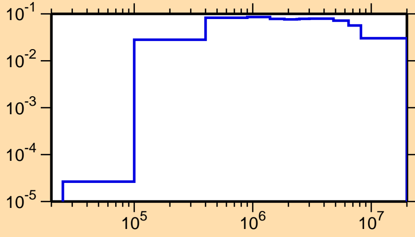
\sigma vs. E for ^{177}\text{Pt}(n,n_2)
