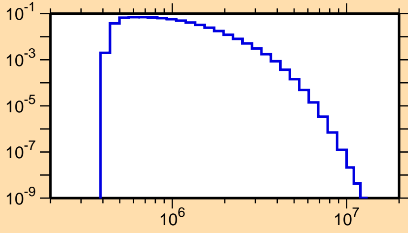
\sigma vs. E for ^{178}\text{Pt}(n,n_2)
