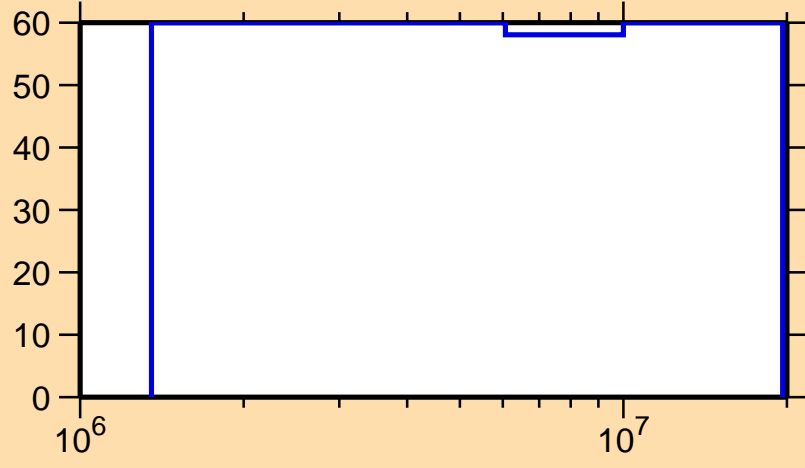
\Delta\sigma/\sigma vs. E for ^{178}\text{Pt}(n,ncont.)
