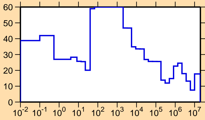
\Delta\sigma/\sigma vs. E for ^{178}\text{Pt}(n,\text{tot.})
