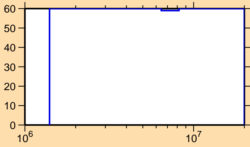
\Delta\sigma/\sigma vs. E for ^{178}\text{Pt}(n,n\text{cont.})
