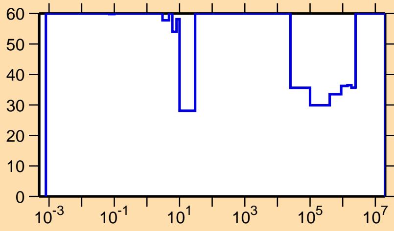
\Delta\sigma/\sigma vs. E for ^{178}\text{Pt}(n,\gamma)
