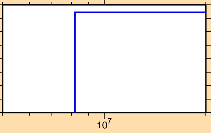
\sigma vs. E for ^{178}\text{Pt}(n,\text{pt})
