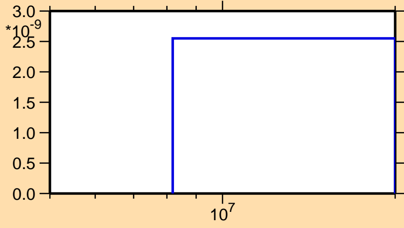
\sigma vs. E for ^{178}\text{Pt}(\text{mt117})
