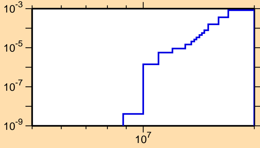
\sigma vs. E for ^{179}\text{Pt}(n,2n\alpha)
