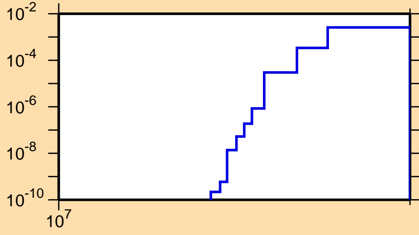
\sigma vs. E for ^{179}\text{Pt}(n,2np)
