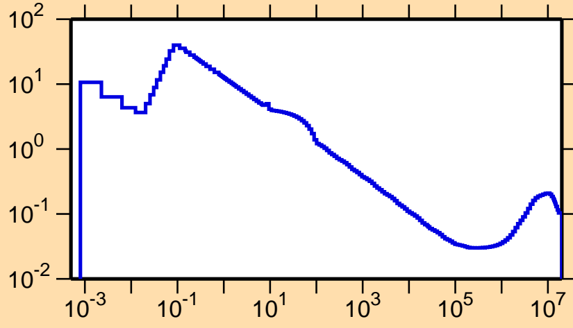
\sigma vs. E for ^{179}\text{Pt}(n,p)
