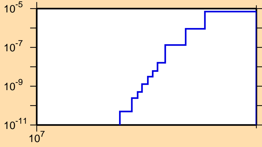
\sigma vs. E for ^{179}\text{Pt}(n,\text{nd})
