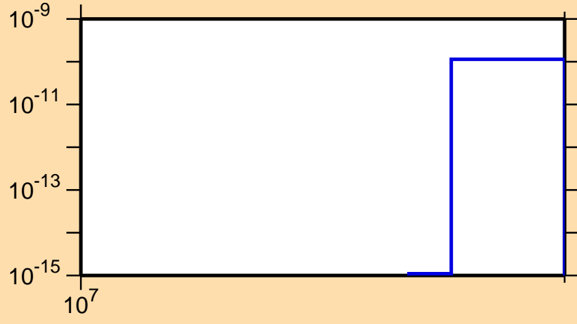
\sigma vs. E for ^{179}\text{Pt}(n,nt)
