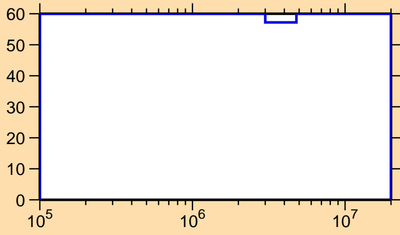
\Delta\sigma/\sigma vs. E for ^{179}\text{Pt}(n,ncont.)
