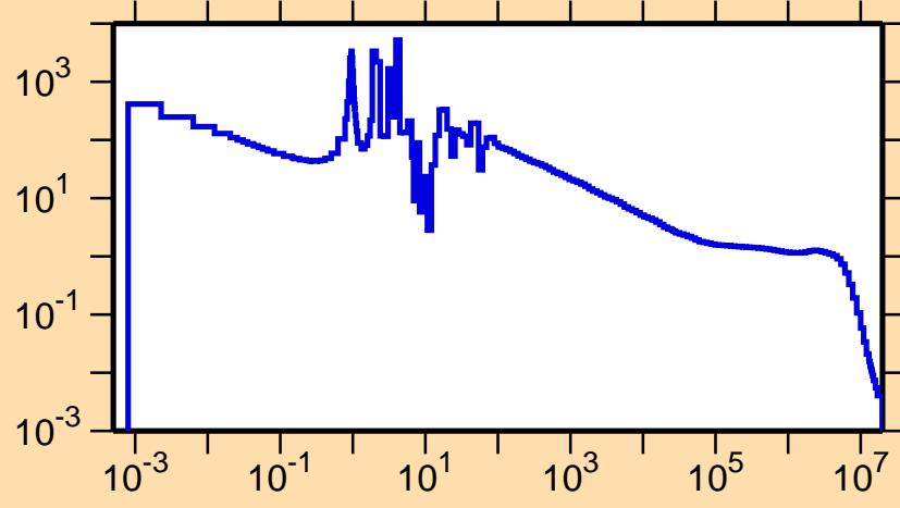
\sigma vs. E for ^{180}\text{Pt}(n,\gamma)
