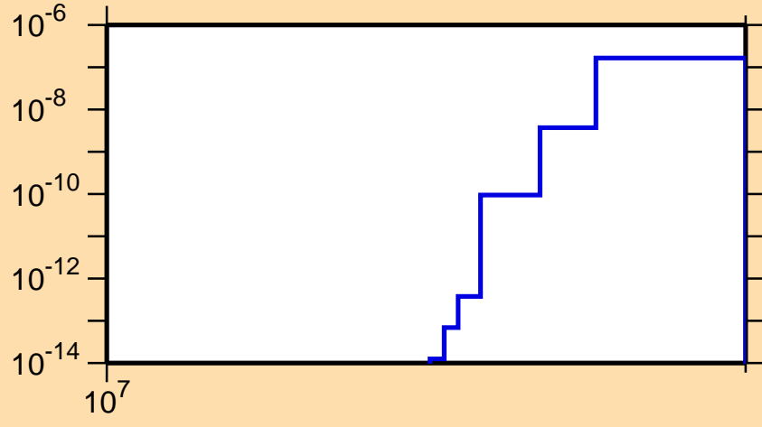
\sigma vs. E for ^{180}\text{Pt}(n,\text{nd})
