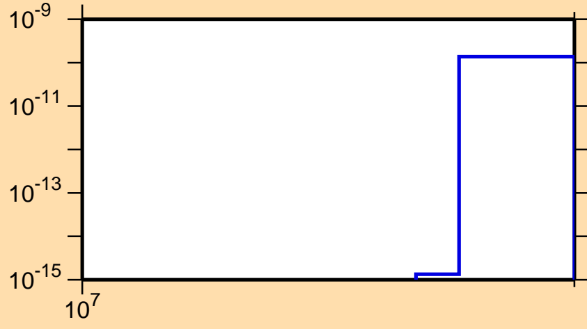
\sigma vs. E for ^{180}\text{Pt}(n,nt)
