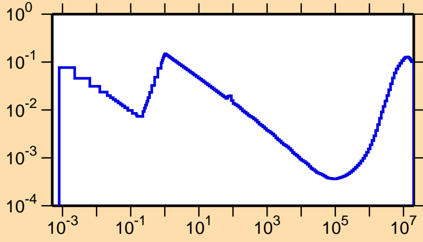
\sigma vs. E for ^{180}\text{Pt}(n,p)
