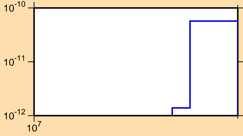
\sigma vs. E for ^{180}\text{Pt}(\text{mt } 34)
