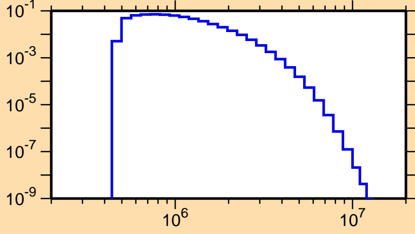
\sigma vs. E for ^{180}\text{Pt}(n,n_3)
