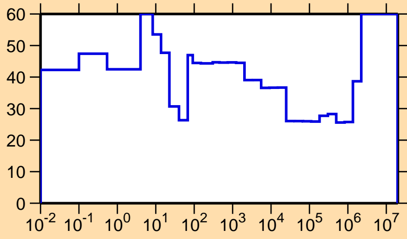
\Delta\sigma/\sigma vs. E for ^{180}\text{Pt}(n,\gamma)
