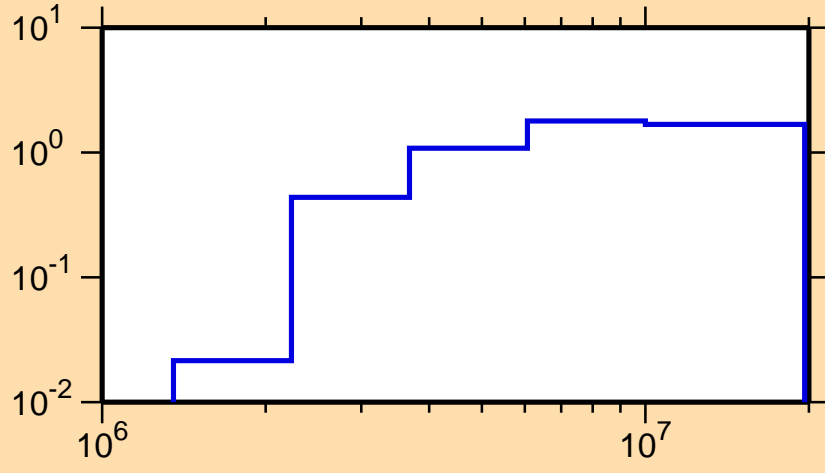
\sigma vs. E for ^{180}\text{Pt}(n,n\text{cont.})
