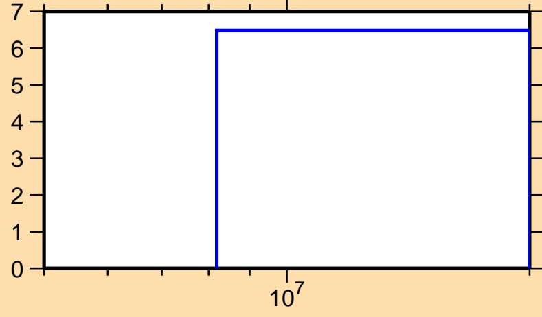
\Delta\sigma/\sigma vs. E for ^{180}\text{Pt}(n,\text{el.})
