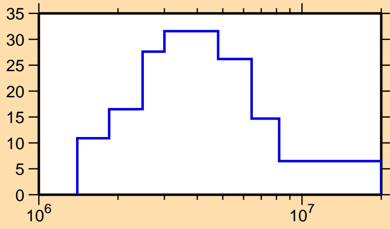
\Delta\sigma/\sigma vs. E for ^{180}\text{Pt}(n, el.)
