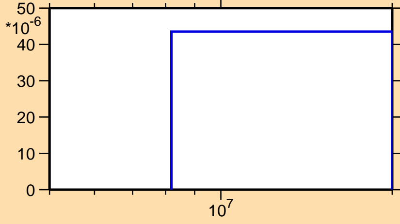
\sigma vs. E for ^{180}\text{Pt}(n,t)
