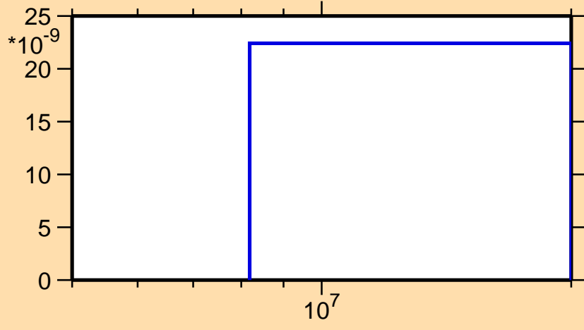
\sigma vs. E for ^{180}\text{Pt}(n,\text{pd})
