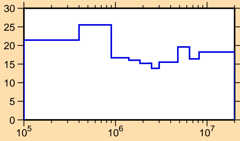
\Delta\sigma/\sigma vs. E for ^{180}\text{Pt}(n,\text{nonel.})
