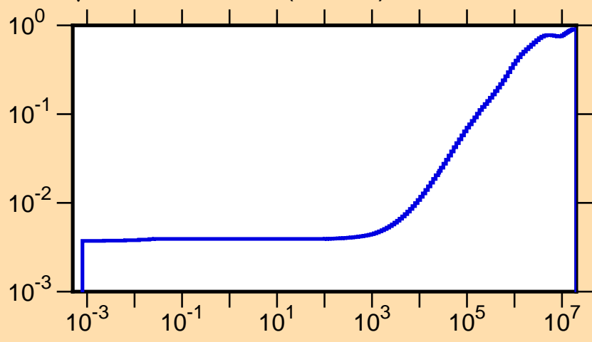
\mu vs. E for ^{181}\text{Pt}(\text{mt251})
