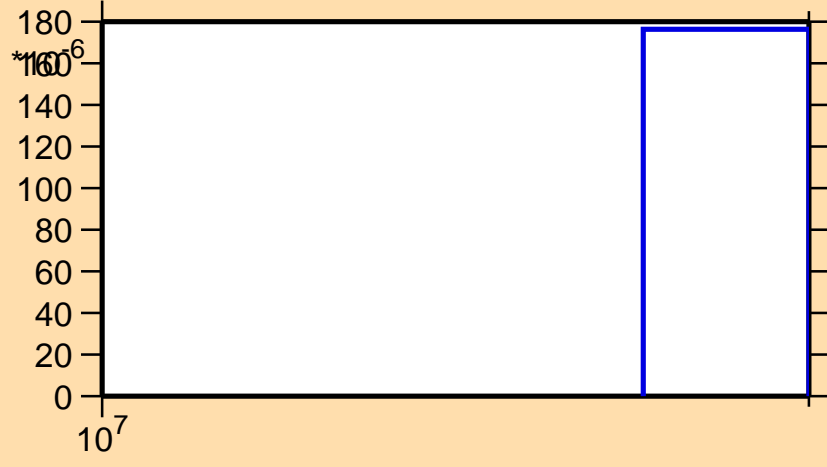
\sigma vs. E for ^{181}\text{Pt}(n,3n)
