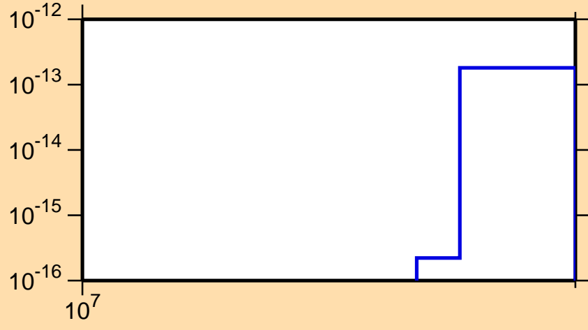
\sigma vs. E for ^{181}\text{Pt}(n,3n\alpha)
