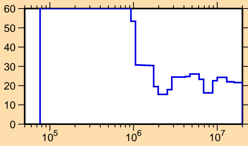
\Delta\sigma/\sigma vs. E for ^{181}\text{Pt}(n,\text{nonel.})
