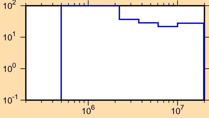
\Delta\sigma/\sigma vs. E for ^{181}\text{Pt}(n,n\text{cont.})
