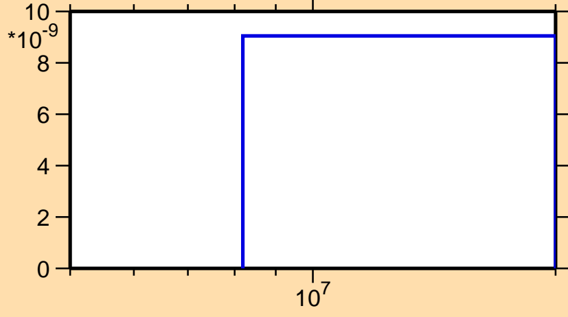
\sigma vs. E for ^{181}\text{Pt}(n,\text{pd})
