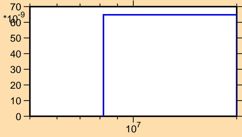
\sigma vs. E for ^{181}\text{Pt}(n,\text{nd})
