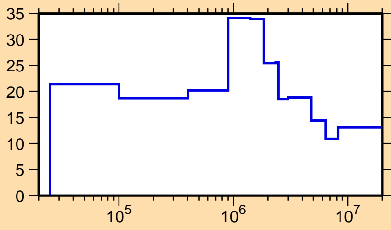
\Delta\sigma/\sigma vs. E for ^{181}\text{Pt}(n,\text{tot.})
