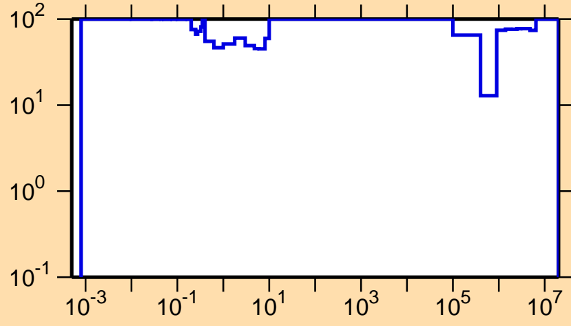
\Delta\sigma/\sigma vs. E for ^{181}\text{Pt}(n,\gamma)
