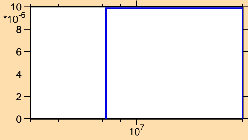
\sigma vs. E for ^{181}\text{Pt}(n,2np)
