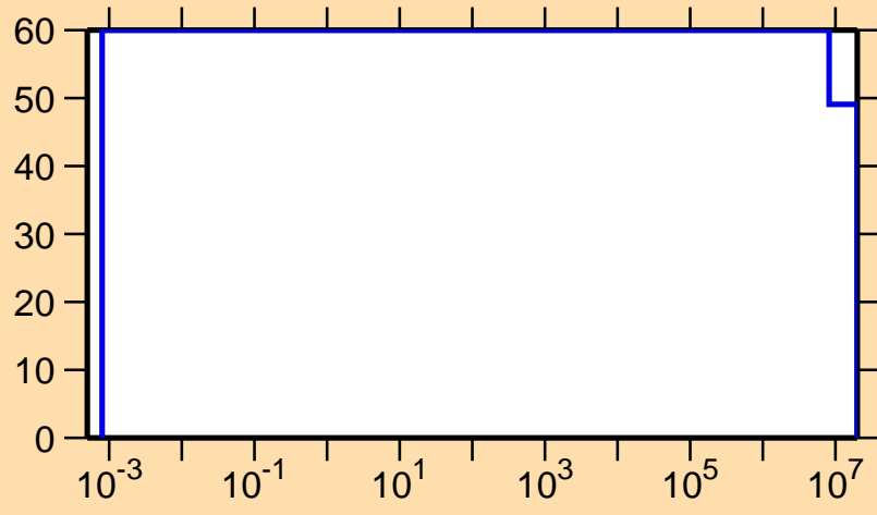
\Delta\sigma/\sigma vs. E for ^{181}\text{Pt}(n,p)
