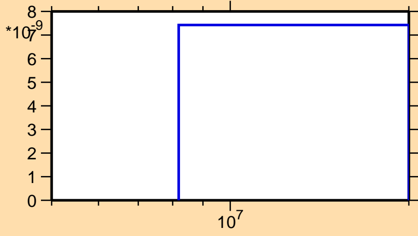
\sigma vs. E for ^{181}\text{Pt}(\text{mt } 45)
