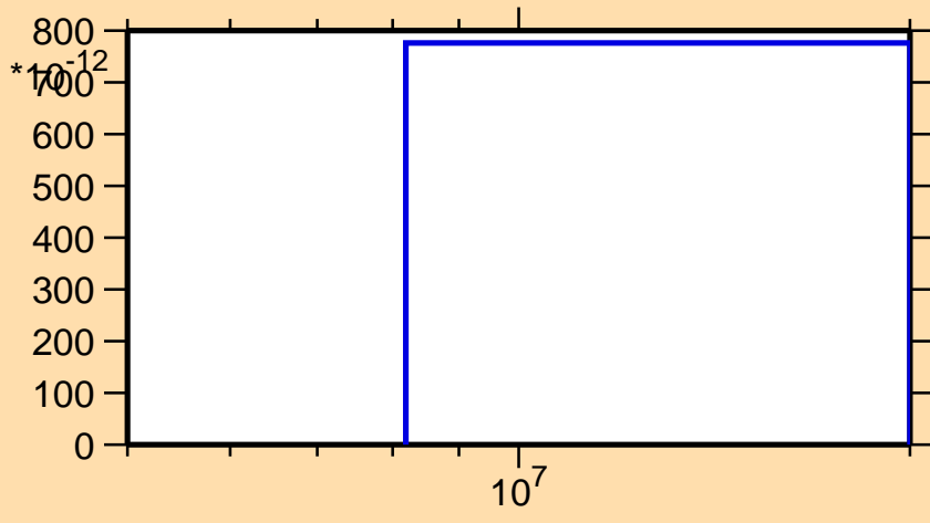
\sigma vs. E for ^{181}\text{Pt}(n,\text{pt})
