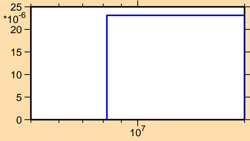
\sigma vs. E for ^{181}\text{Pt}(n,2n\alpha)
