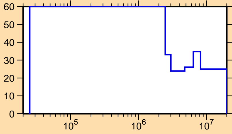
\Delta\sigma/\sigma vs. E for ^{181}\text{Pt}(n,n_1)
