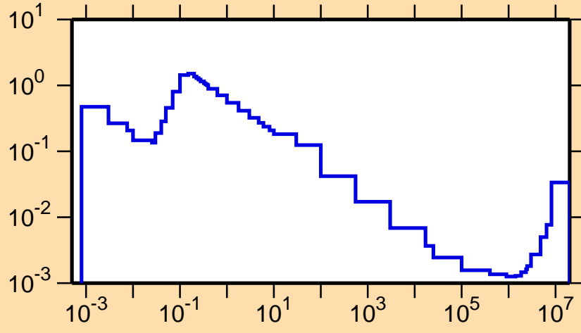
\sigma vs. E for ^{181}\text{Pt}(n,\alpha)
