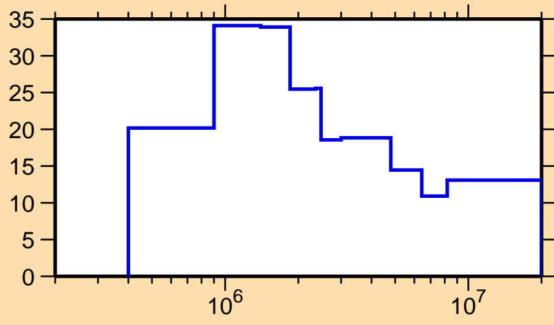
\Delta\sigma/\sigma vs. E for ^{181}\text{Pt}(n,tot.)
