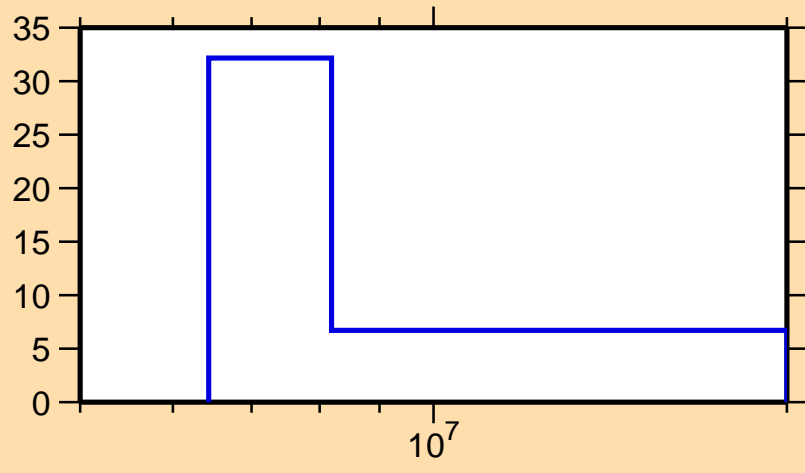
\Delta\sigma/\sigma vs. E for ^{181}\text{Pt}(n,\text{el.})
