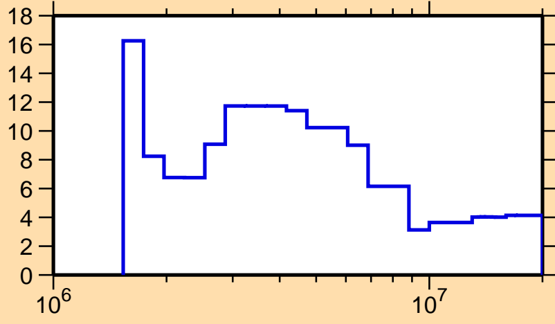
\Delta\sigma/\sigma vs. E for ^{182}\text{Pt}(n, tot.)
