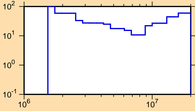
\Delta\sigma/\sigma vs. E for ^{182}\text{Pt}(n,n\text{cont.})
