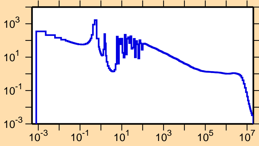
\sigma vs. E for ^{182}\text{Pt}(n,\gamma)
