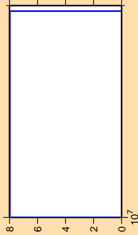
\Delta\sigma/\sigma vs. E for ^{182}\text{Pt}(n,\text{pt})
