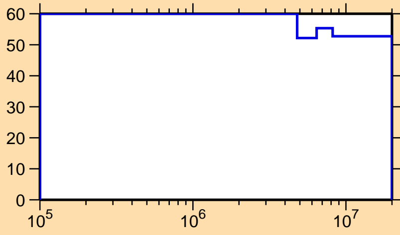
\Delta\sigma/\sigma vs. E for ^{182}\text{Pt}(n,n_1)
