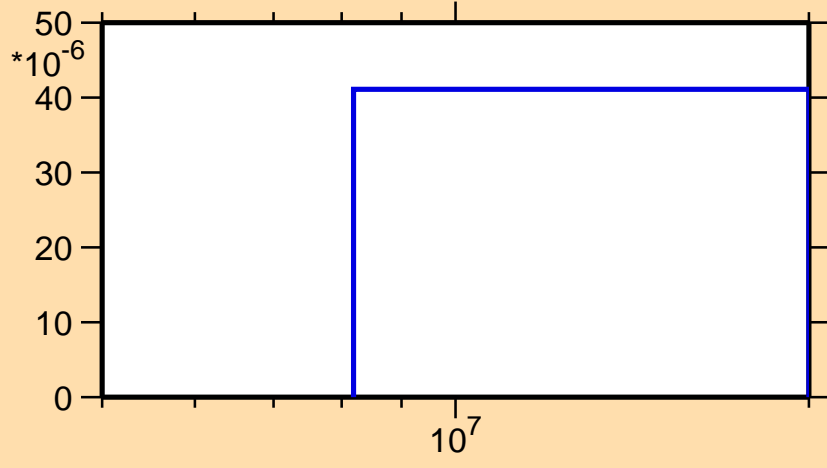
\sigma vs. E for ^{182}\text{Pt}(n,t)
