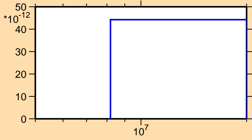
\sigma vs. E for ^{182}\text{Pt}(\text{mt117})
