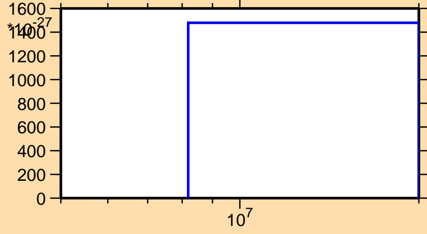
\sigma vs. E for ^{182}\text{Pt}(\text{mt } 11)
