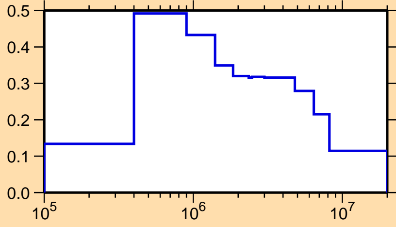
\sigma vs. E for ^{182}\text{Pt}(n,n_1)
