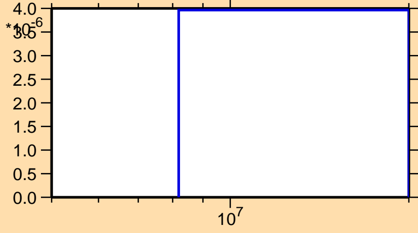
\sigma vs. E for ^{182}\text{Pt}(n,3n)
