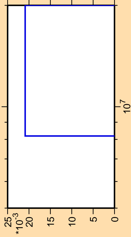
\Delta\sigma/\sigma vs. E for ^{182}\text{Pt}(n,3n\alpha)
