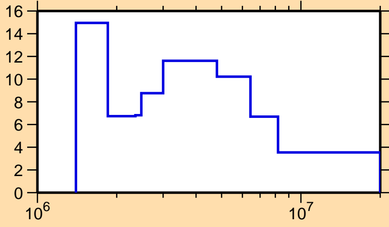
\Delta\sigma/\sigma vs. E for ^{182}\text{Pt}(n,\text{tot.})
