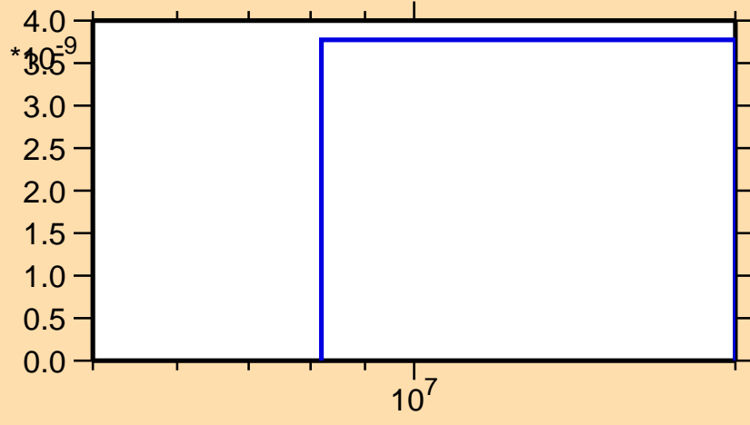
\sigma vs. E for ^{182}\text{Pt}(\text{mt } 45)
