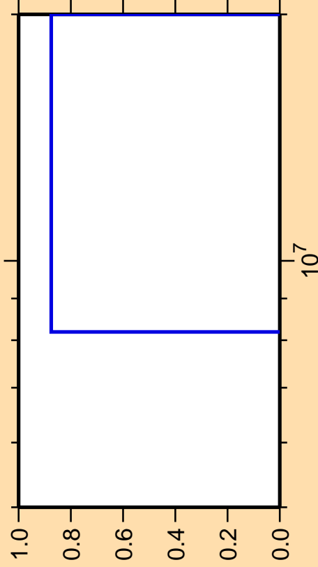
\Delta\sigma/\sigma vs. E for ^{182}\text{Pt}(\text{mt } 34)
