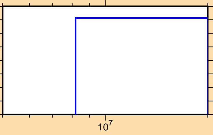
\sigma vs. E for ^{182}\text{Pt}(n,nt)
