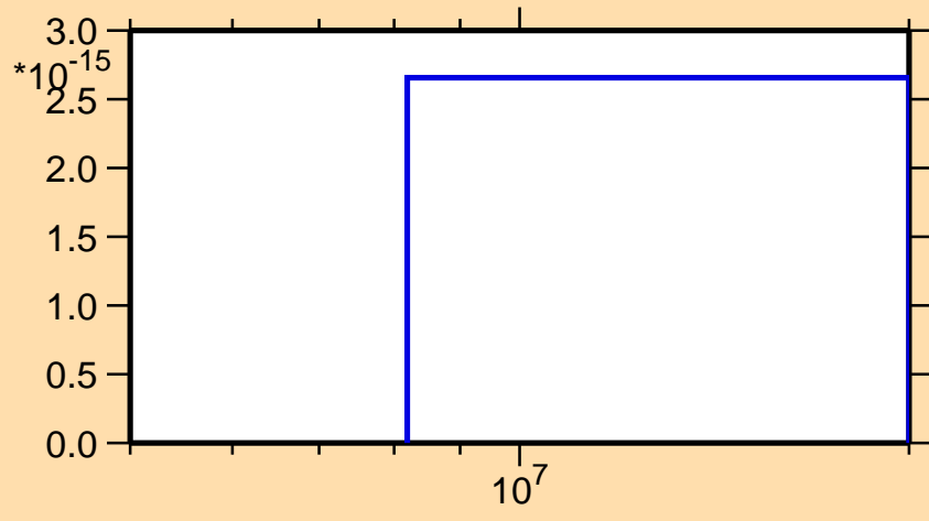
\sigma vs. E for ^{182}\text{Pt}(n,3n\alpha)
