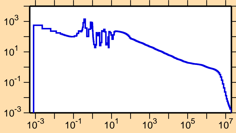
\sigma vs. E for ^{183}\text{Pt}(n,\gamma)
