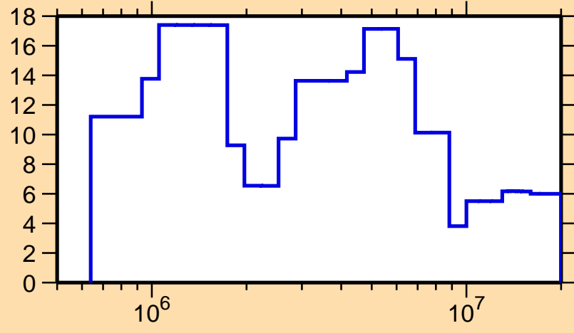
\Delta\sigma/\sigma vs. E for ^{183}\text{Pt}(n, el.)
