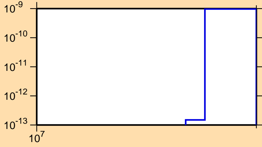
\sigma vs. E for ^{183}\text{Pt}(n,nt)
