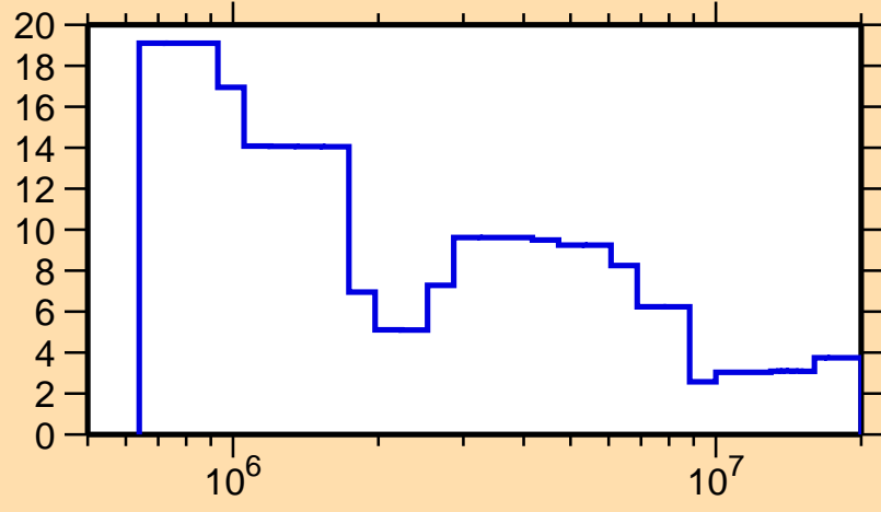
\Delta\sigma/\sigma vs. E for ^{183}\text{Pt}(n,tot.)
