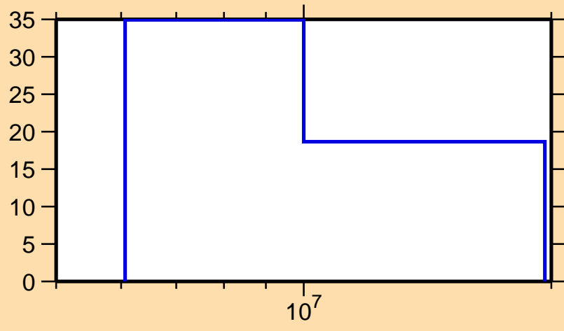
\Delta\sigma/\sigma vs. E for ^{183}\text{Pt}(n,2n)
