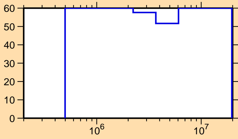
\Delta\sigma/\sigma vs. E for ^{183}\text{Pt}(n,n_1)
