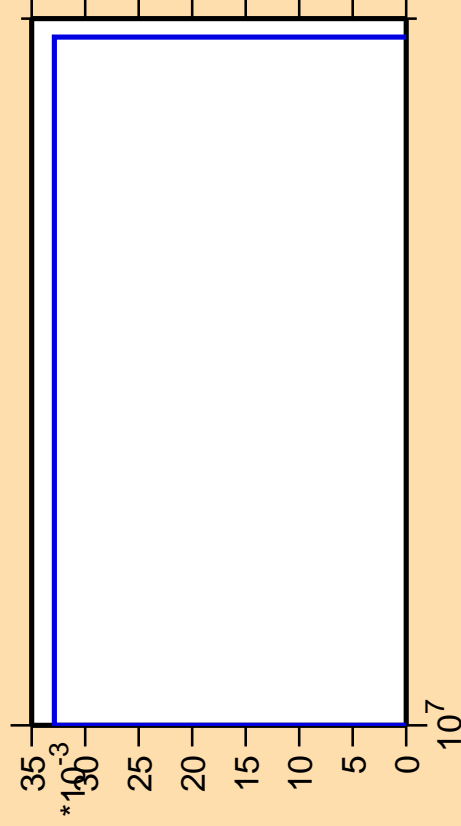
\Delta\sigma/\sigma vs. E for ^{183}\text{Pt}(n,3n\alpha)
