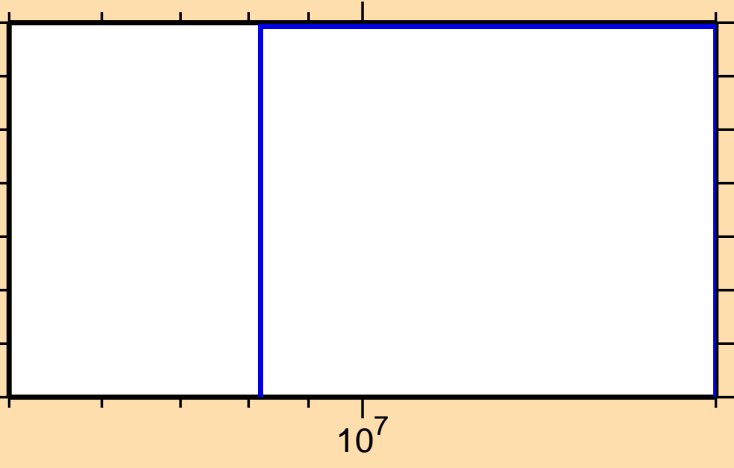
\sigma vs. E for ^{183}\text{Pt}(n,2n\alpha)
