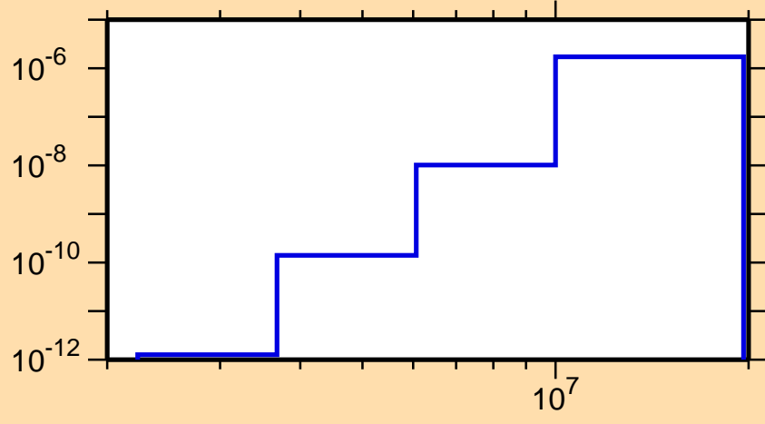
\sigma vs. E for ^{183}\text{Pt}(n,p\alpha)
